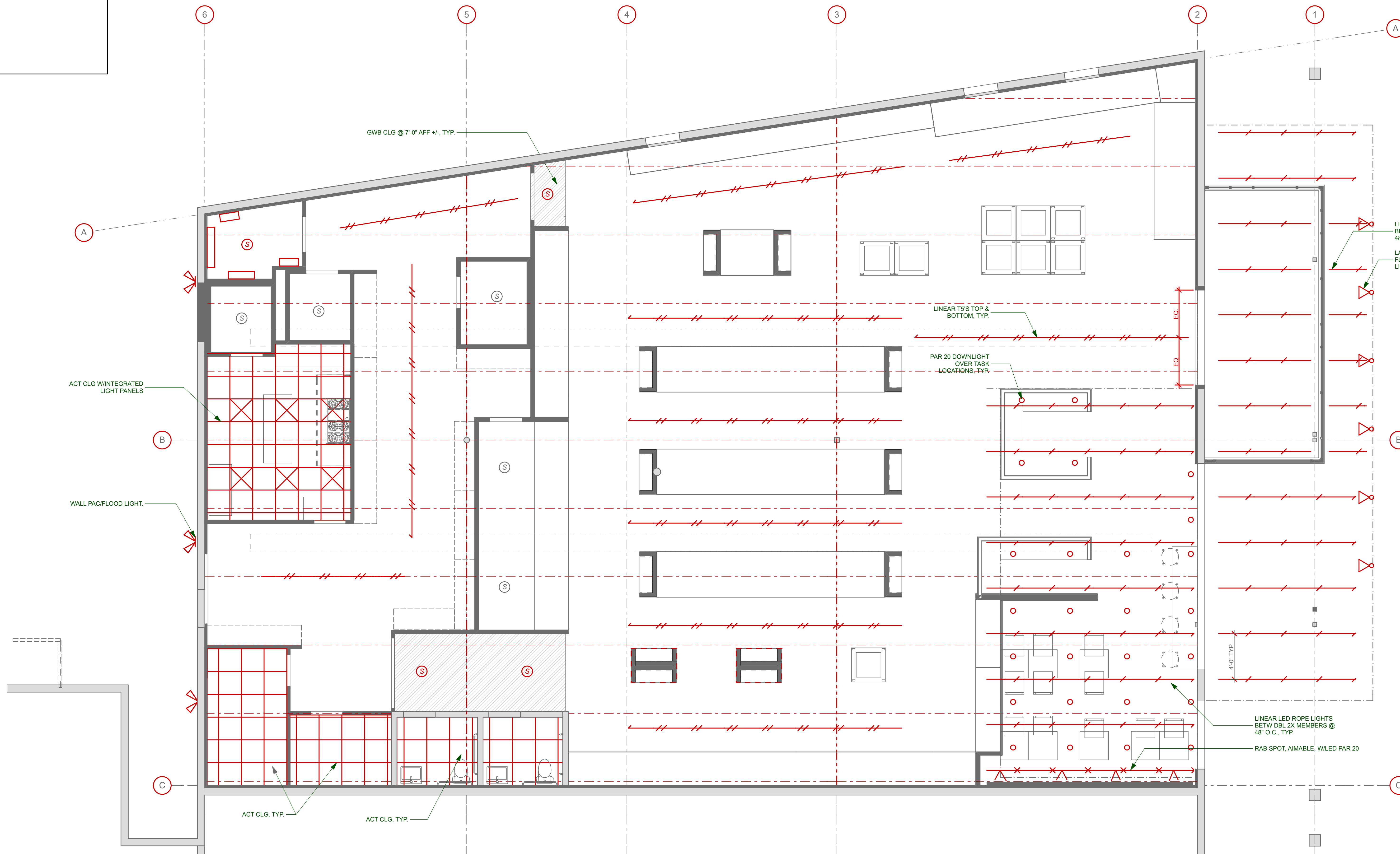
1 MAIN LEVEL RCP SCALE: 1/4" = 1'-0"
