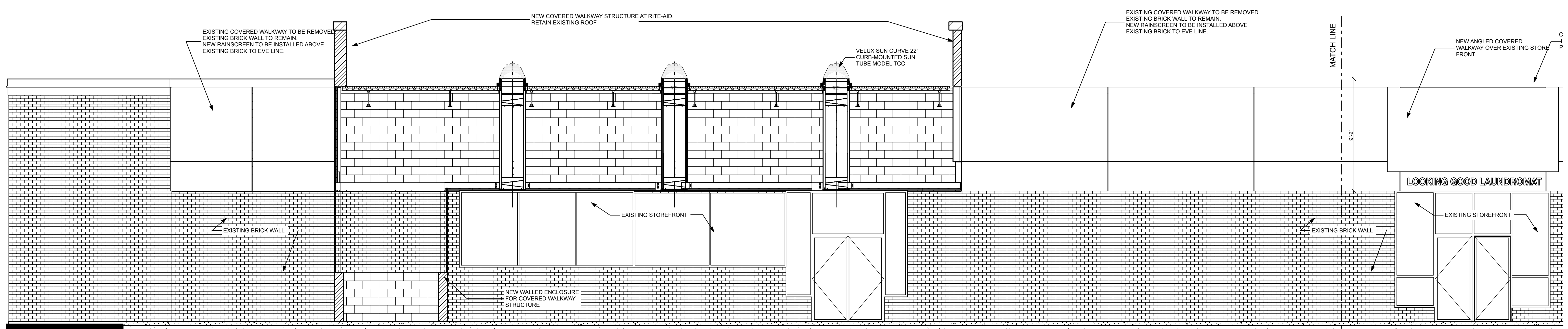
1 SECTION AT LENGTH OF COVERED WALKWAY SCALE: 1/4" = 1'-0"
