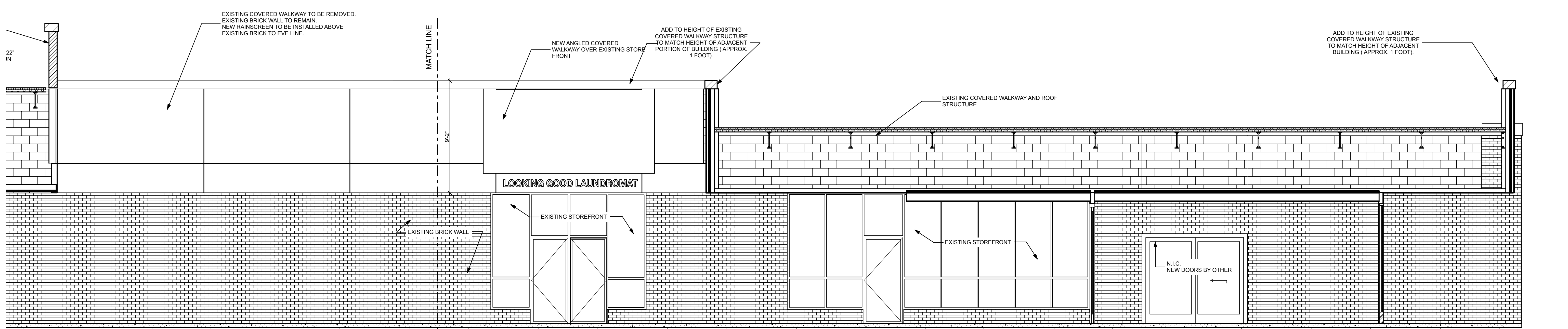
2 SECTION AT LENGTH OF COVERED WALKWAY SCALE: 1/4" = 1'-0"
