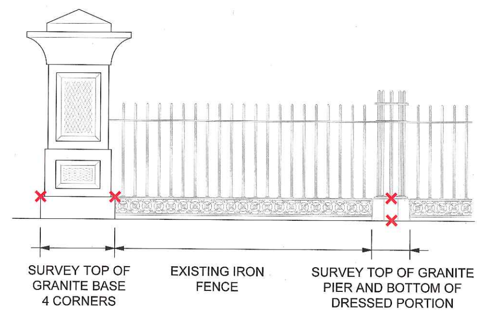
2 SPOT GRADE SURVEY ELEVATION AT CONGRESS ST - BASE BID S-03 1/2" = 1'-0" (ON 22 X 34 SHEET)
