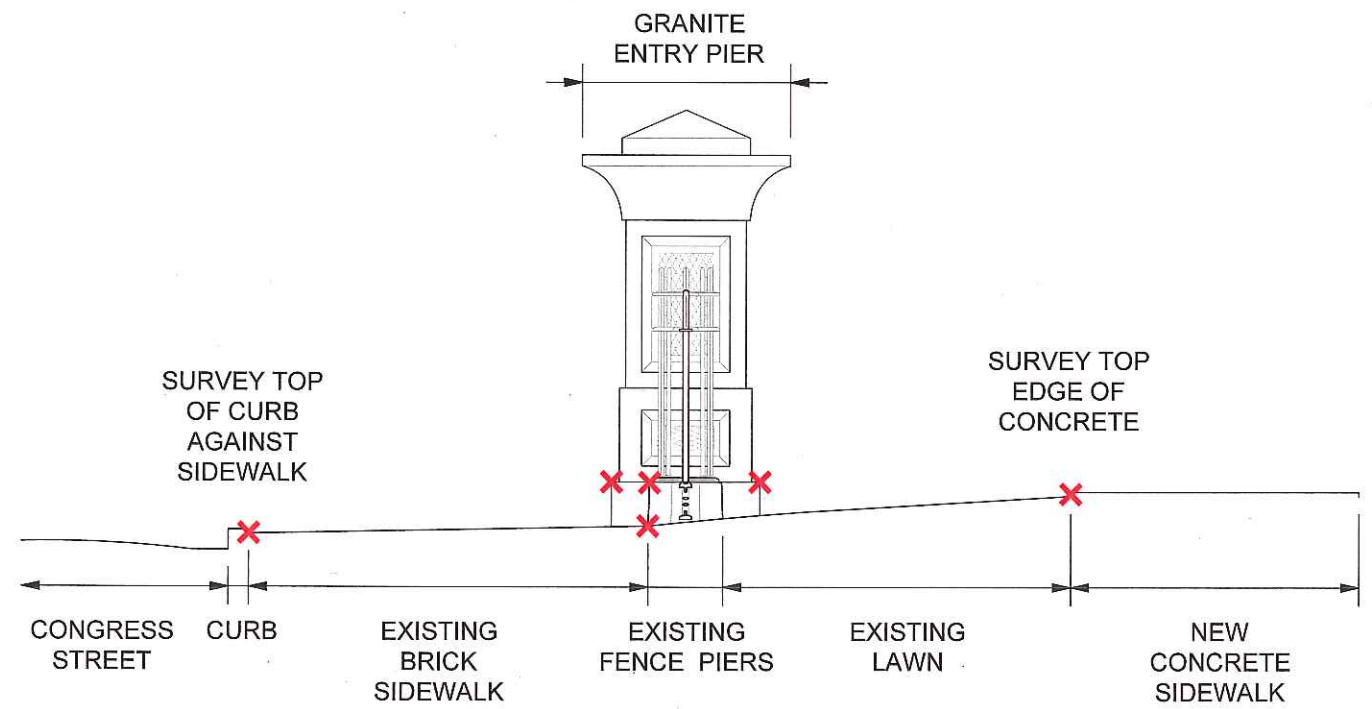
3 SPOT GRADE SURVEY SITE SECTION - BASE BID S-03 1/2" = 1'-0" (ON 22 X 34 SHEET)
