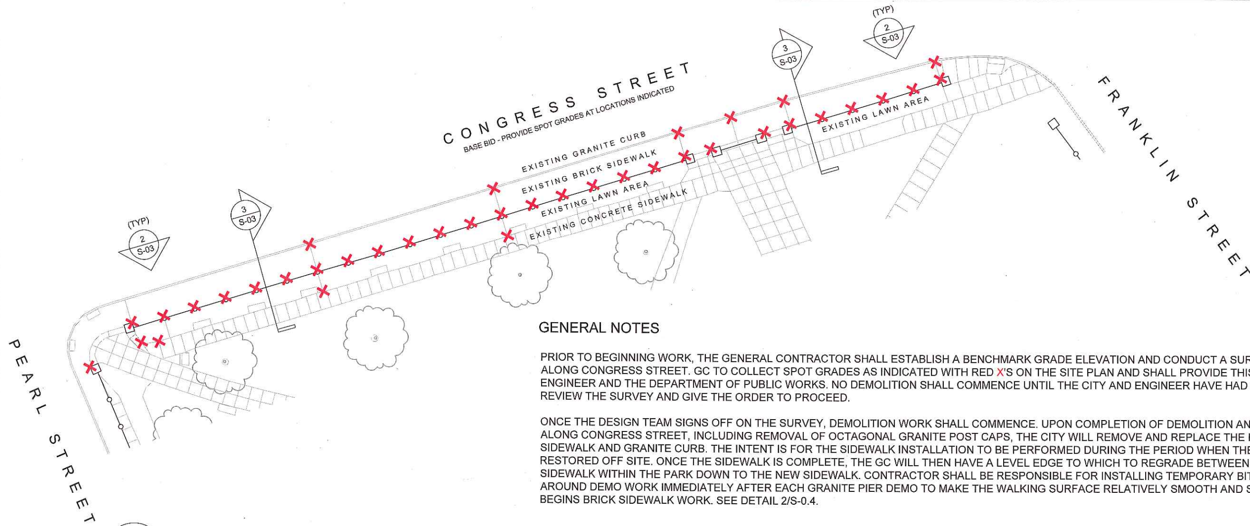
1 SPOT GRADE SURVEY PLAN OF EXISTING CONDITIONS- BASE BID S-03 1" = 16'-0" (ON 22 X 34 SHEET)
