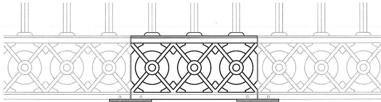
4 ELEVATION OF NEW ORNAMENTAL BOTTOM RAIL S2.5 3" = 1'-0" (ON 22 X 34 SHEET)
