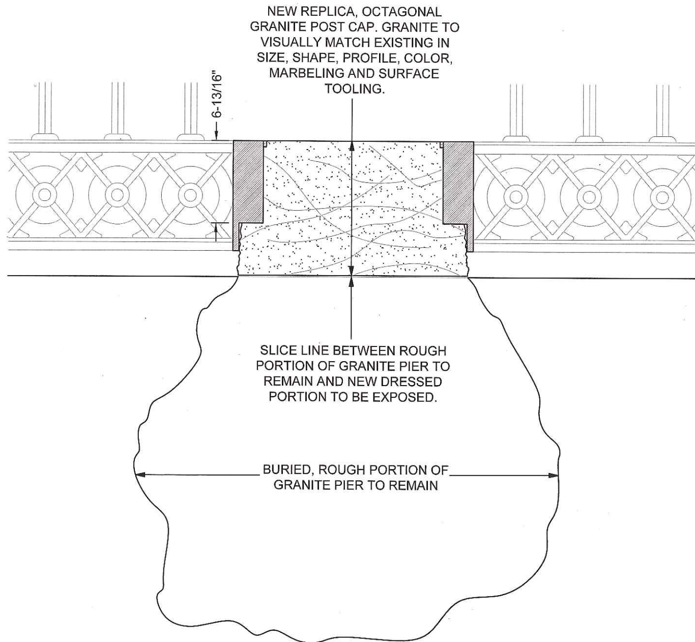
2 SECTION DETAIL AT NEW GRANITE POST CAP S2.3 3" = 1'-0" (ON 22 X 34 SHEET)
