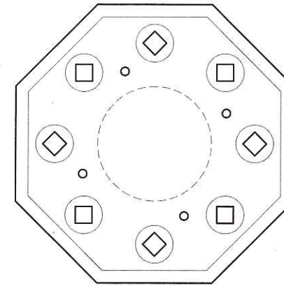
3 TOP VIEW OF GRANITE POST CAP AND NEW IRON CASTING PLATE S2.3 3" = 1'-0" (ON 22 X 34 SHEET)
