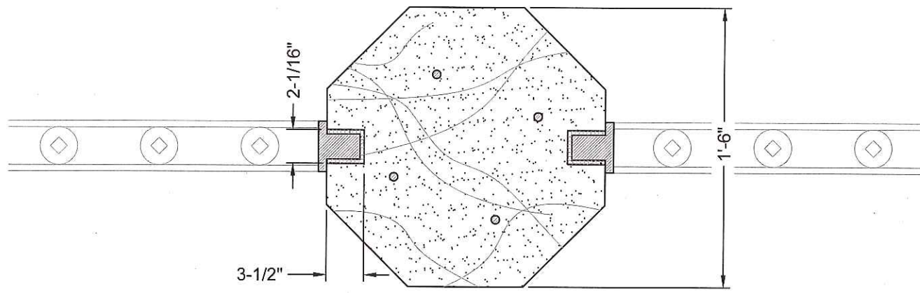
1 TOP VIEW OF GRANITE POST CAP S2.3 3" = 1'-0" (ON 22 X 34 SHEET)
