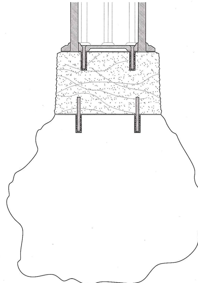
4 SECTION DETAIL AT NEW GRANITE POST CAP AND CASTING S2.3 3" = 1'-0" (ON 22 X 34 SHEET)
