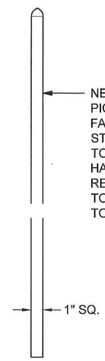
13 S2.2 MILD STEEL SHAPE TYPE 6 ELEV. OF FENCE POST PICKET 3" = 1'-0" (ON 22 X 34 SHEET)
