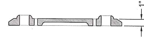
8 S2.2 CASTING TYPE 3 TOP VIEW OF FENCE POST BASE CASTING 3" = 1'-0" (ON 22 X 34 SHEET)
