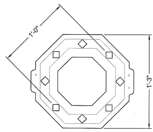
9 S2.2 CASTING TYPE 4 TOP VIEW OF FENCE POST BASE CASTING 3" = 1'-0" (ON 22 X 34 SHEET)
