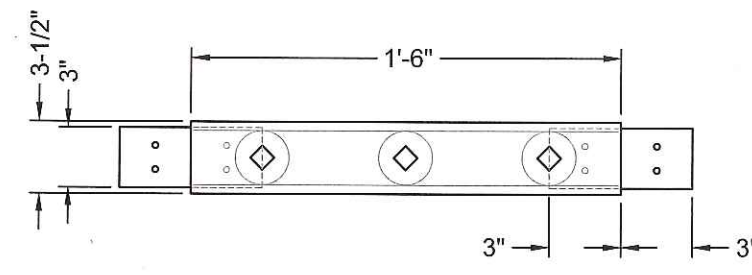
4 S2.2 CASTING TYPE 2 TOP VIEW OF BOTTOM RAIL CASTING 3" = 1'-0" (ON 22 X 34 SHEET)
