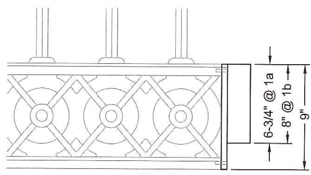
1 S2.2 CASTING TYPES 1a and 1b ELEVATION OF BOTTOM RAIL TAB CASTING 3" = 1'-0" (ON 22 X 34 SHEET)
