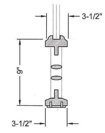
6 S2.2 CASTING TYPE 2 SECTION OF BOTTOM RAIL CASTING 3" = 1'-0" (ON 22 X 34 SHEET)
