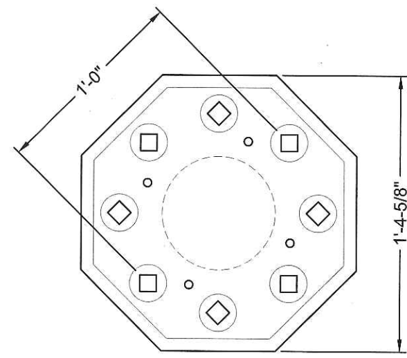
7 S2.2 CASTING TYPE 3 TOP VIEW OF FENCE POST BASE CASTING 3" = 1'-0" (ON 22 X 34 SHEET)
