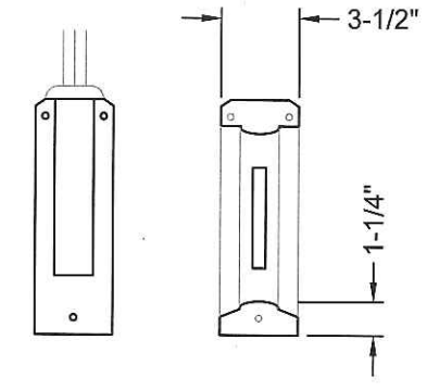
3 S2.2 CASTING TYPES 1a and 1b SIDES OF TAB CASTING 3" = 1'-0" (ON 22 X 34 SHEET)
