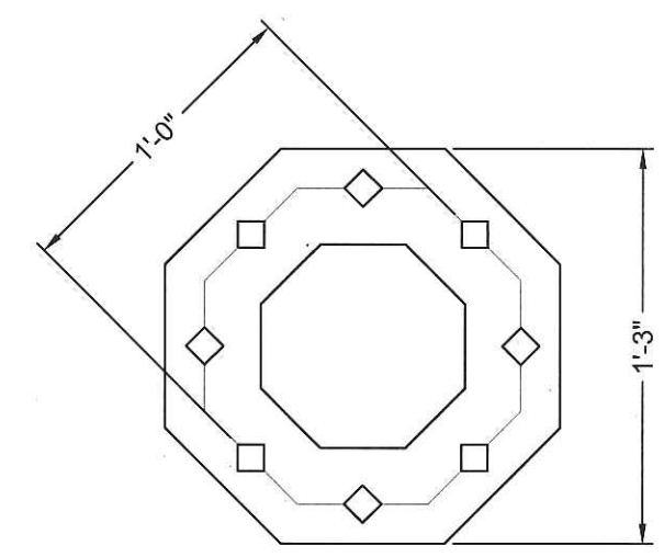
11 S2.2 CASTING TYPE 5 TOP VIEW OF FENCE POST BASE CASTING 3" = 1'-0" (ON 22 X 34 SHEET)
