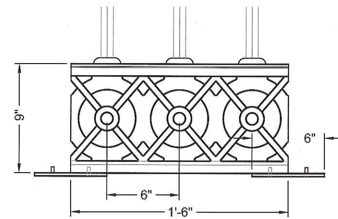
5 S2.2 CASTING TYPE 2 ELEVATION OF ORNAMENTAL BOTTOM RAIL CASTING 3" = 1'-0" (ON 22 X 34 SHEET)
