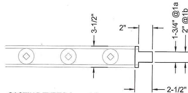
1 S2.2 CASTING TYPES 1a and 1b ELEVATION OF BOTTOM RAIL TAB CASTING 3" = 1'-0" (ON 22 X 34 SHEET)
