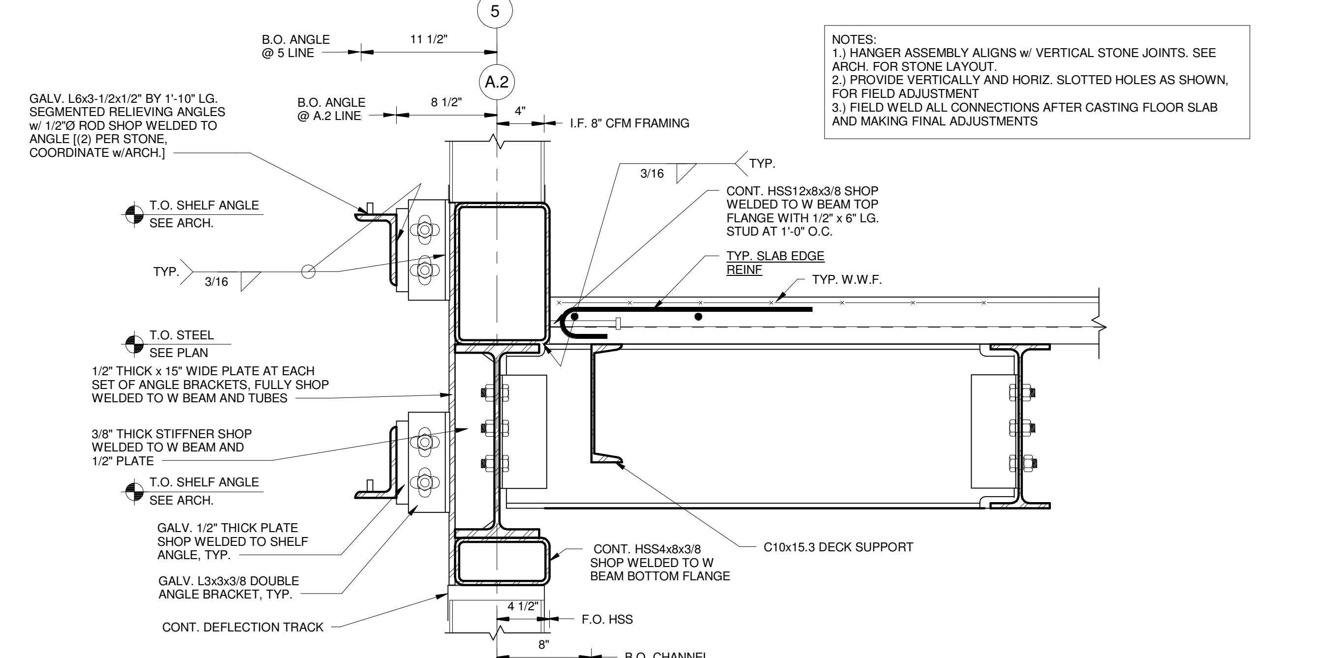
E8 SECTION 1 1/2" = 1'-0"
