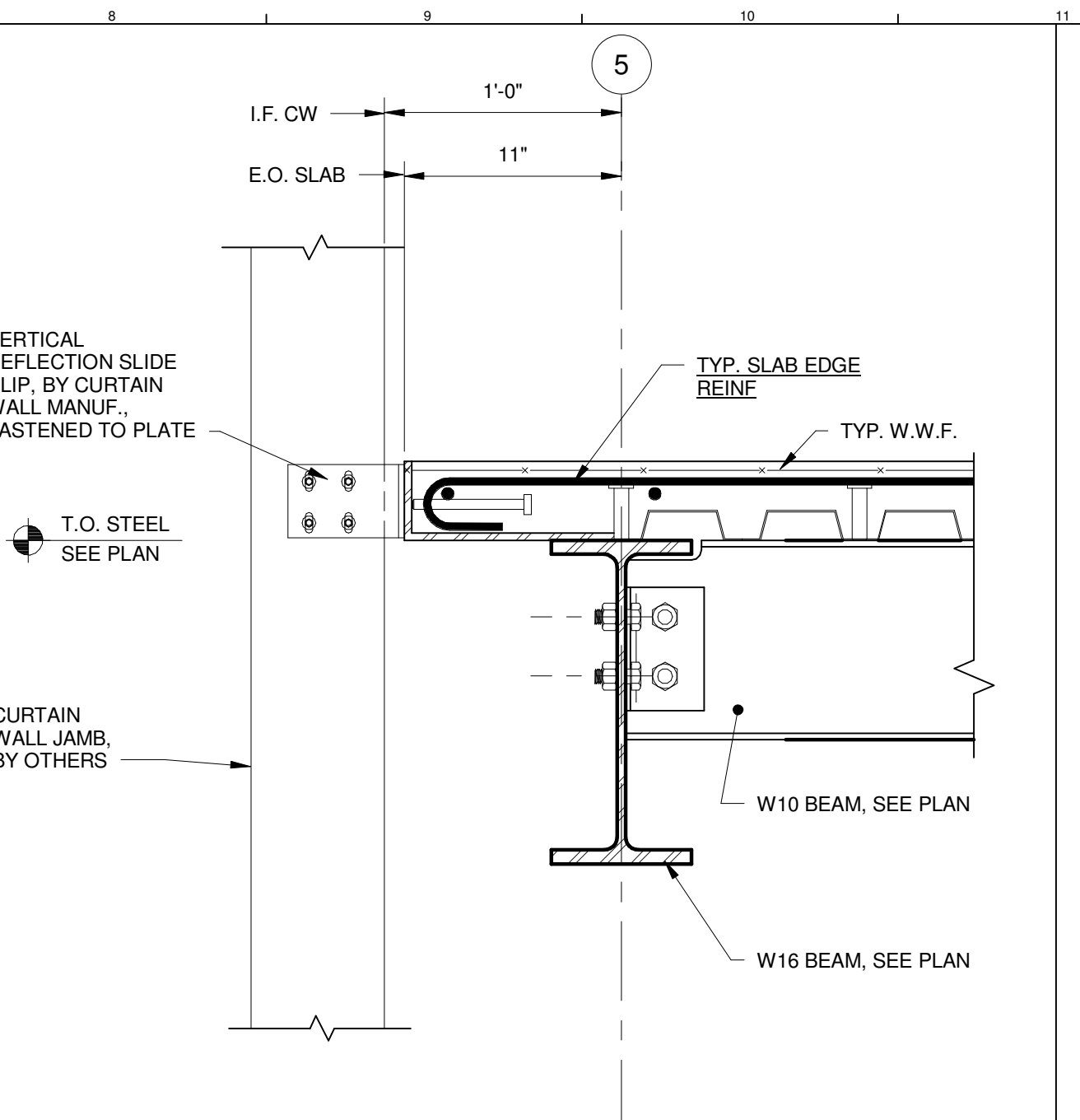
K8 SECTION 1 1/2" = 1'-0"
