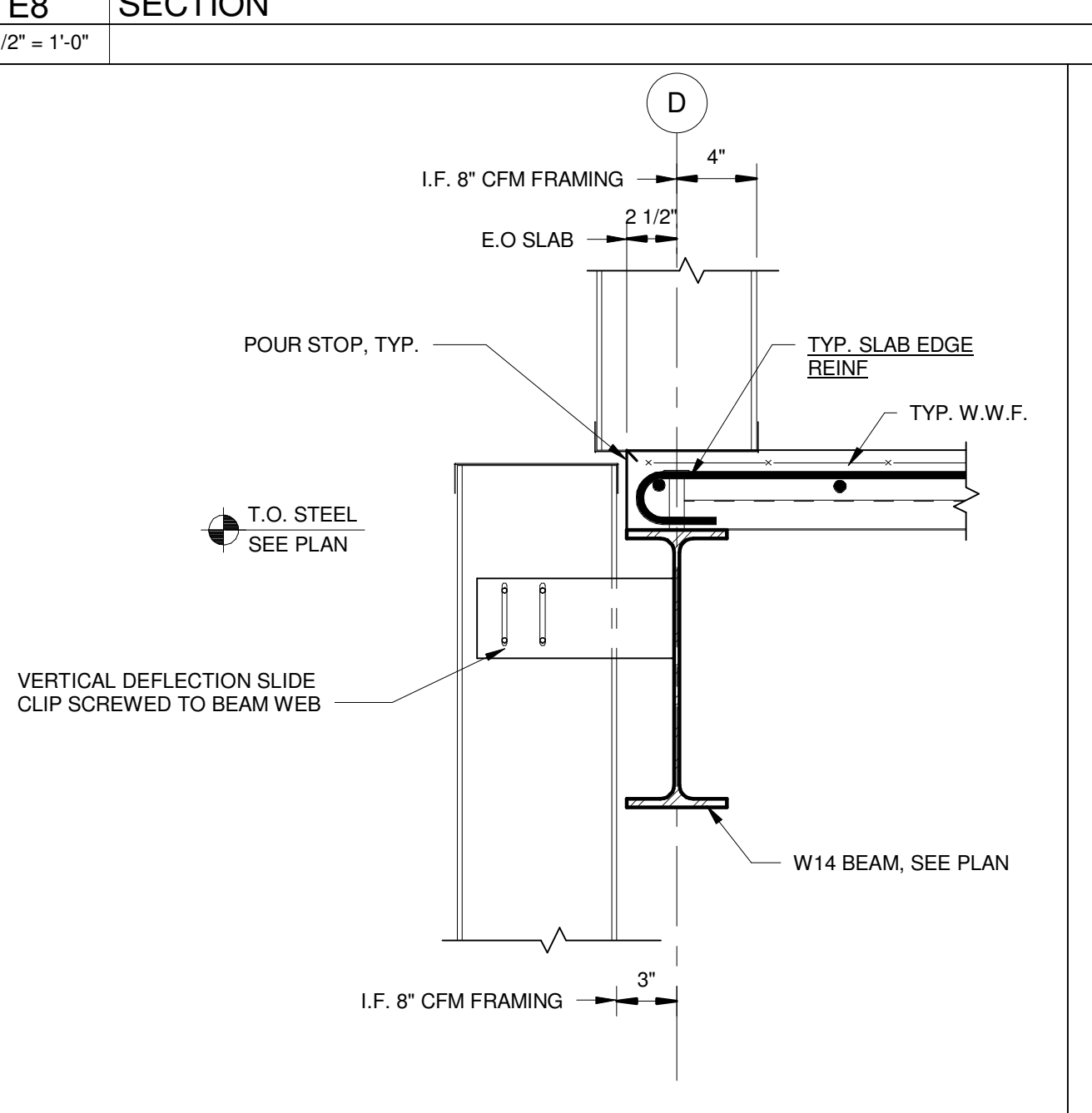
A8 SECTION 1 1/2" = 1'-0"
