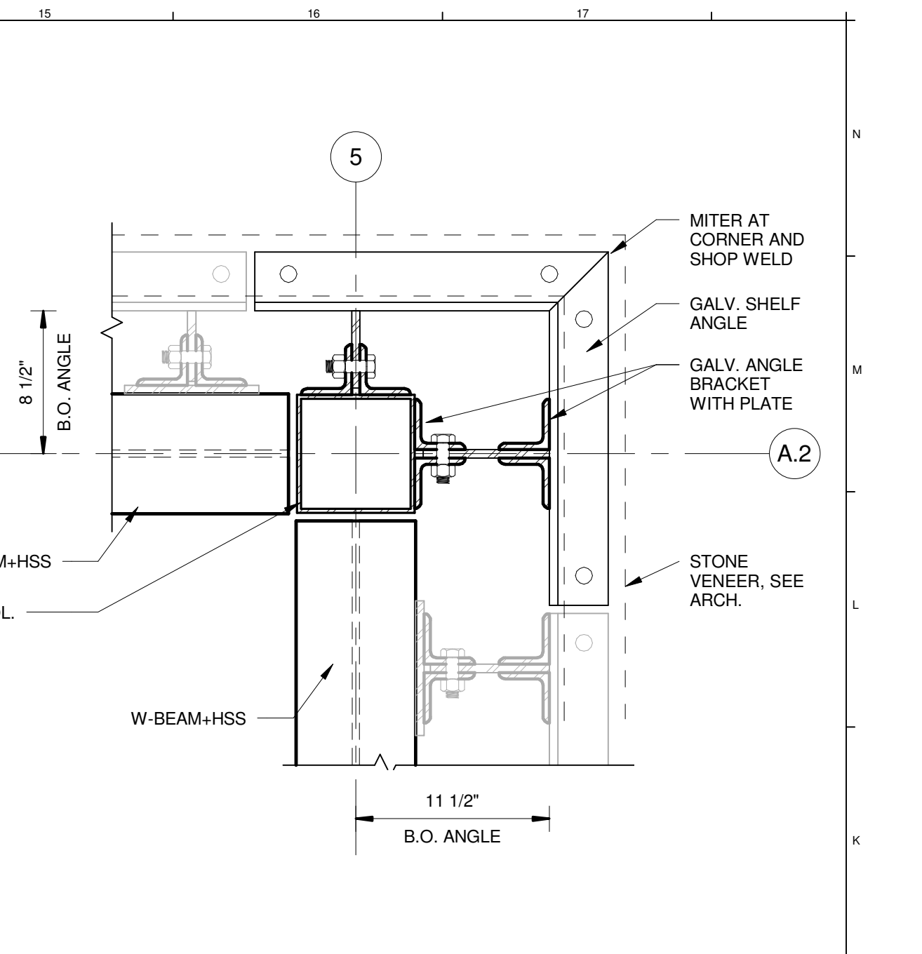
K14 PLAN DETAIL 1 1/2" = 1'-0"
