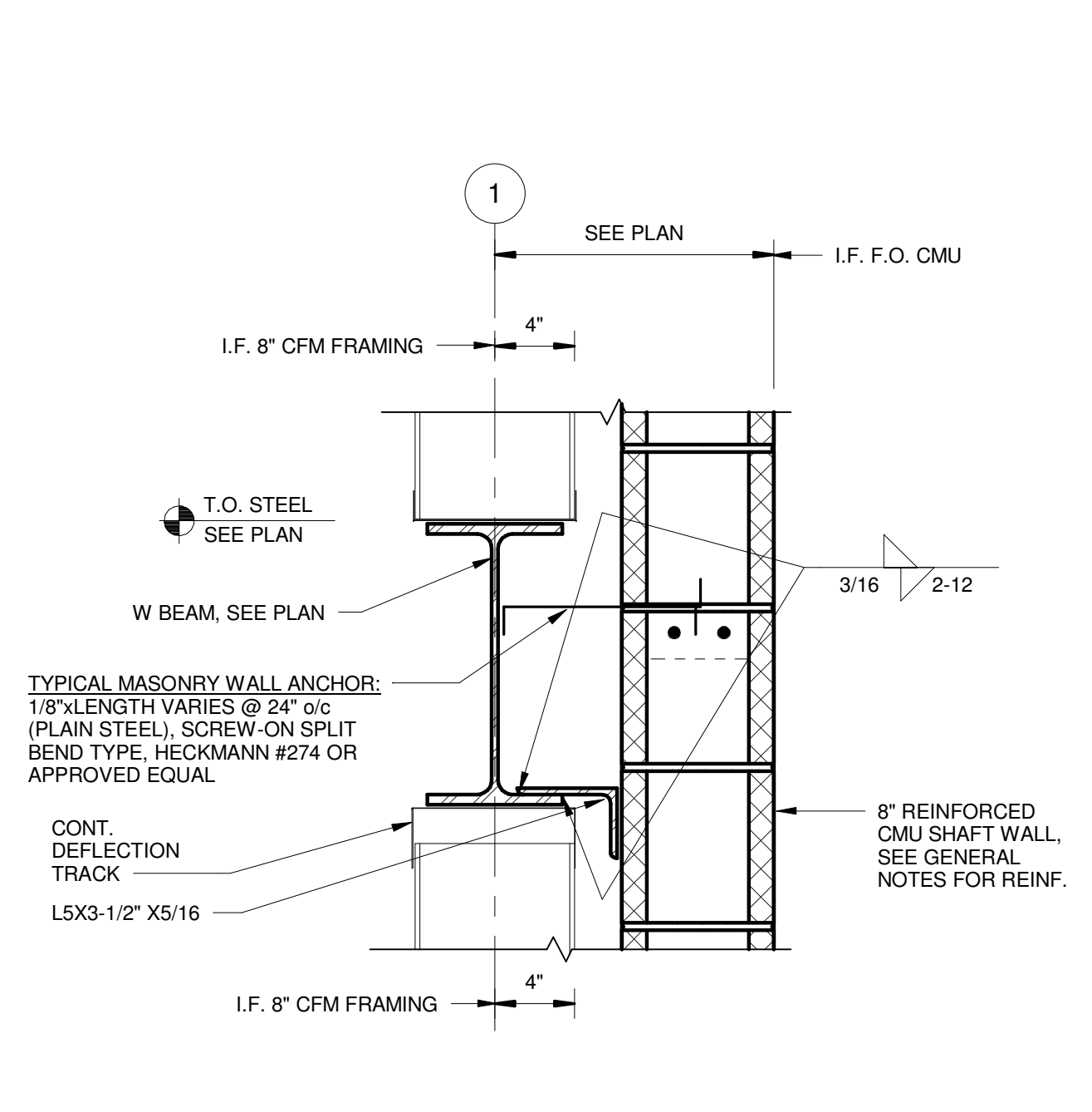
E4 SECTION 1 1/2" = 1'-0"
