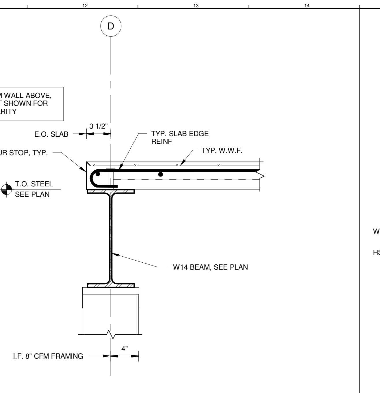
K11 SECTION 1 1/2" = 1'-0"
