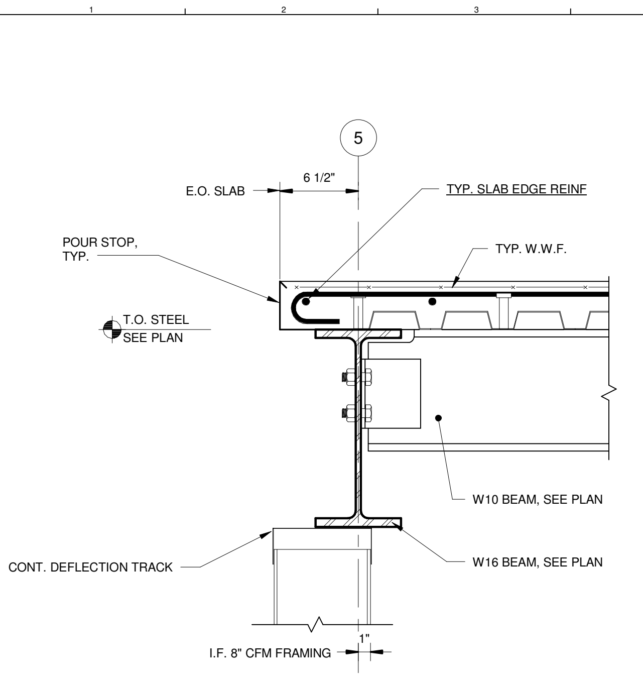
K1 SECTION 1 1/2" = 1'-0"
