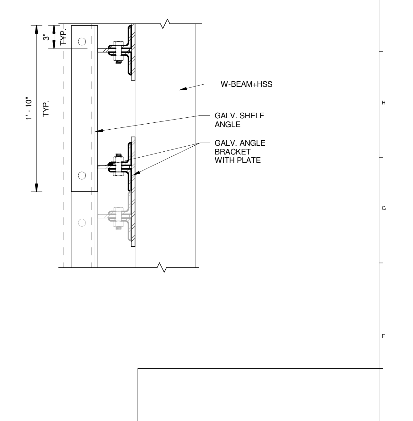
K14 PLAN DETAIL 1 1/2" = 1'-0"
