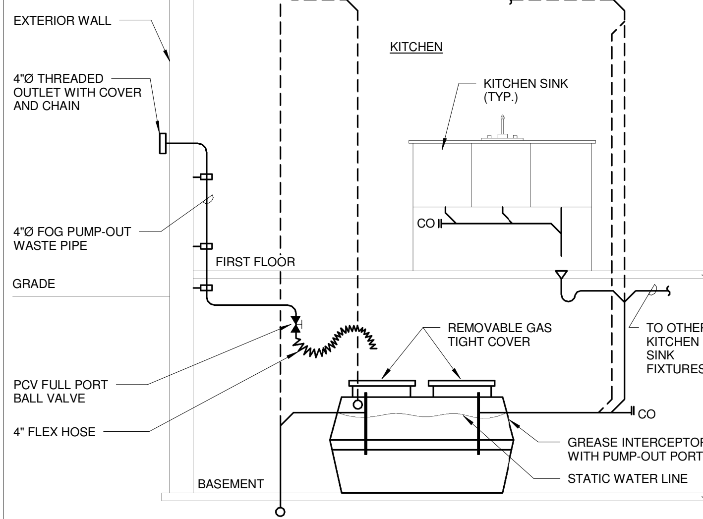
K12 GREASE (F.O.G.) INTERCEPTOR SCHEMATIC NTS
