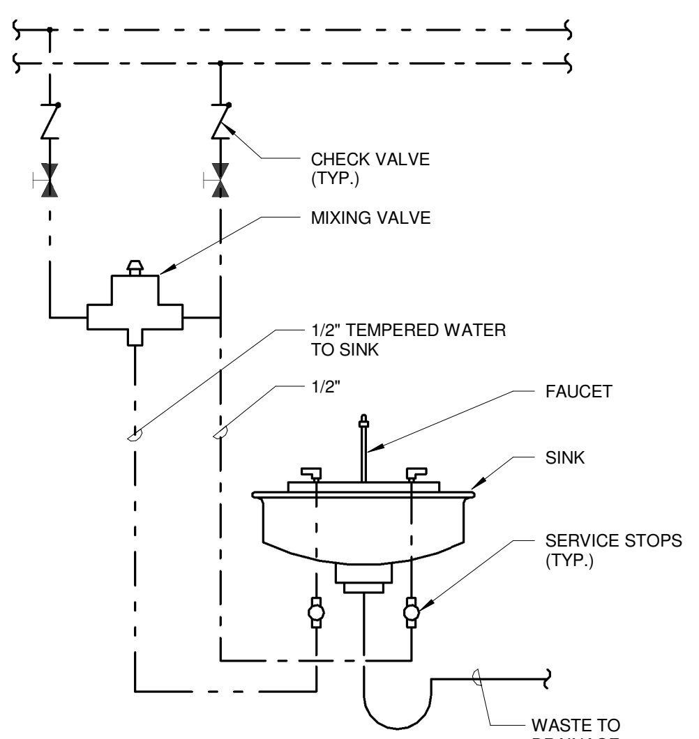
E5 MIXING VALVE PIPING SCHEMATIC NTS
