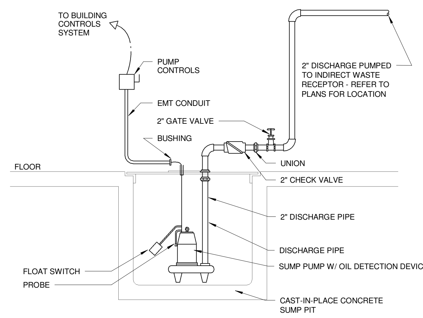
A9 SUMP PUMP DETAIL NTS
