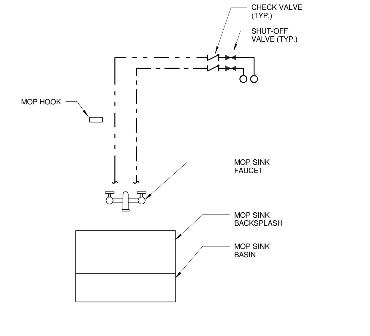
A1 MOP SINK PIPING SCHEMATIC (SERVICE SINK SIM.) NTS
