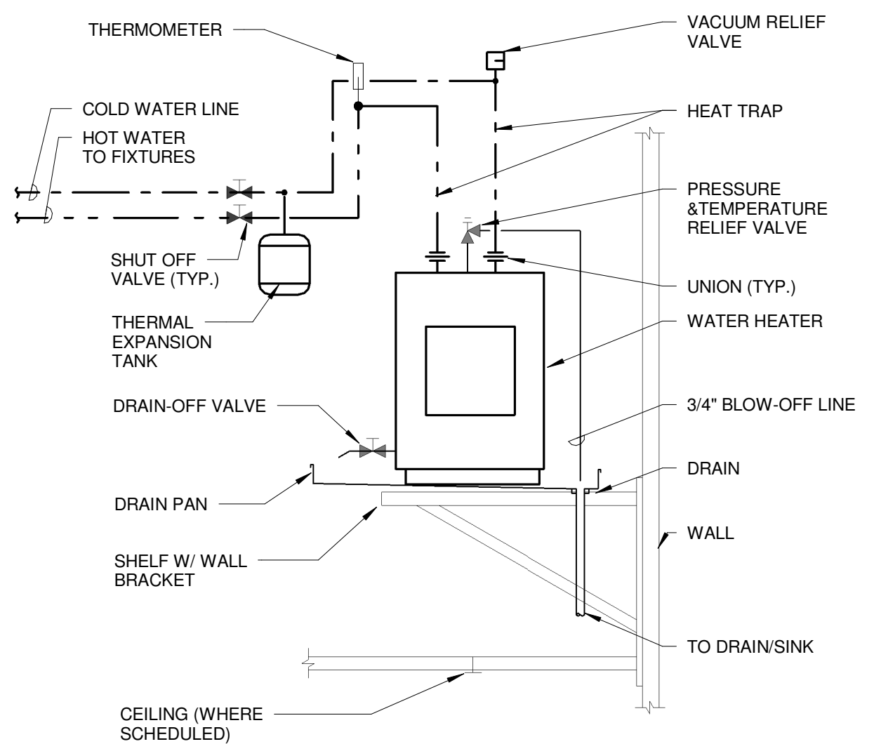
A5 WATER HEATER PIPING SCHEMATIC NTS
