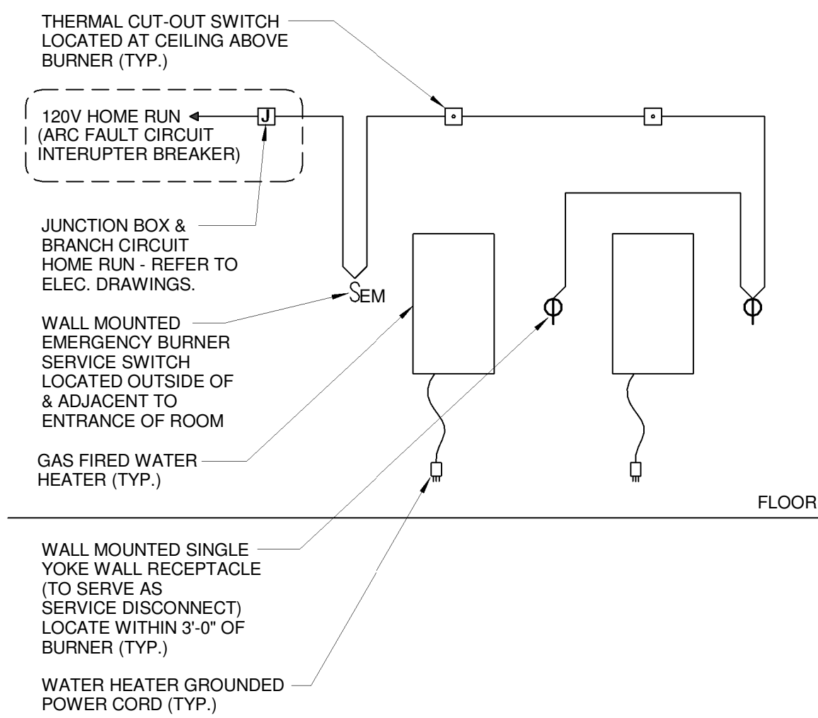
K1 GAS FIRED DOMESTIC WATER HEATING PLANT EMERGENCY & THERMAL SWITCH CONTROLS NTS
