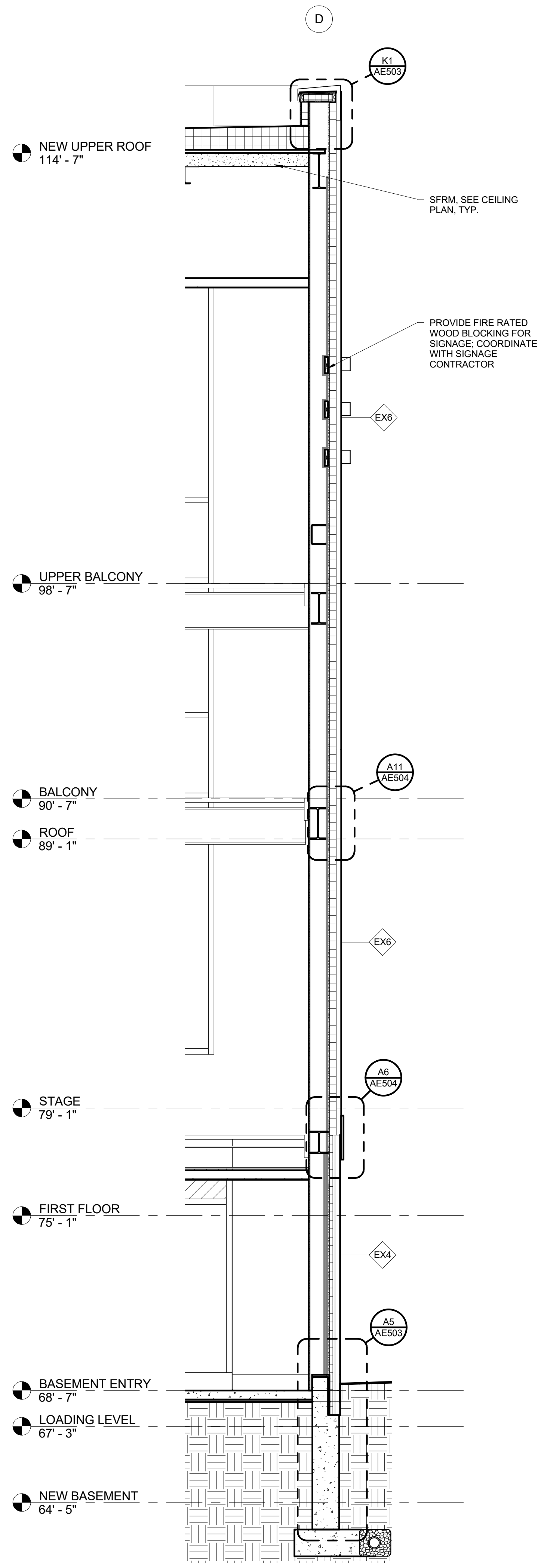
A1 WALL SECTION @ THIN STONE VENEER 3/8" = 1'-0" AE101
