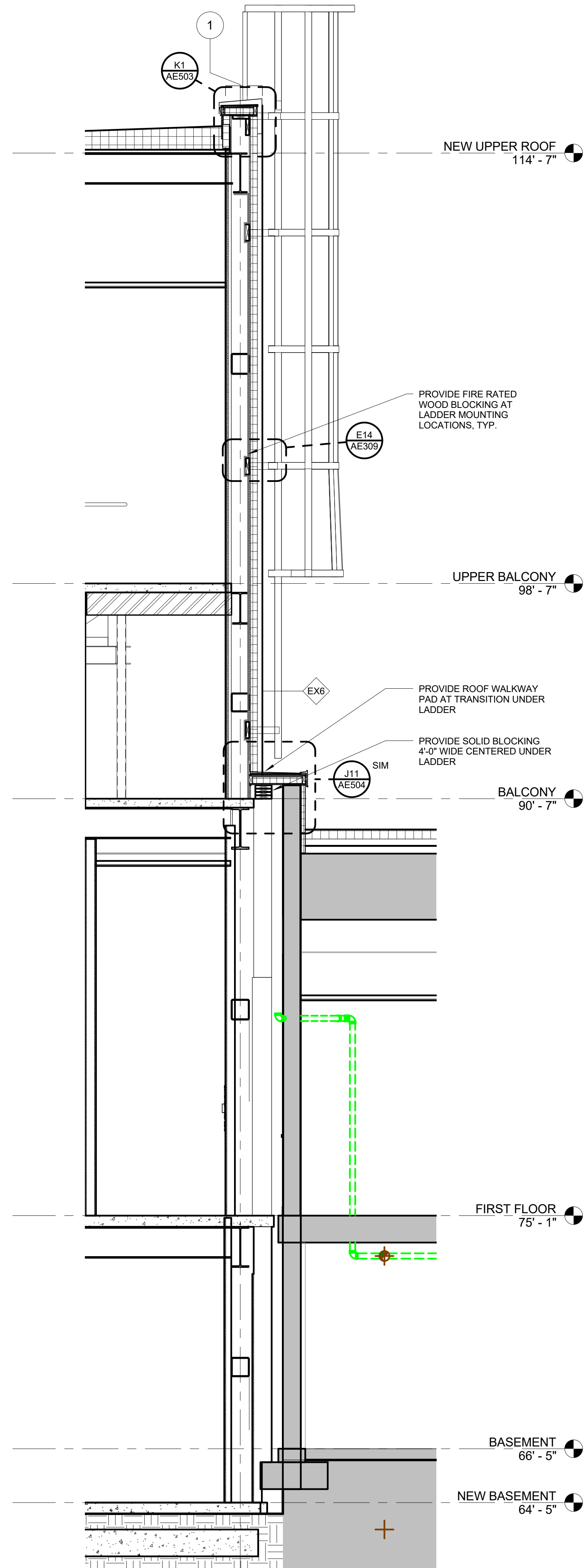
A12 WALL SECTION @ LADDER 3/8" = 1'-0" AE101A
