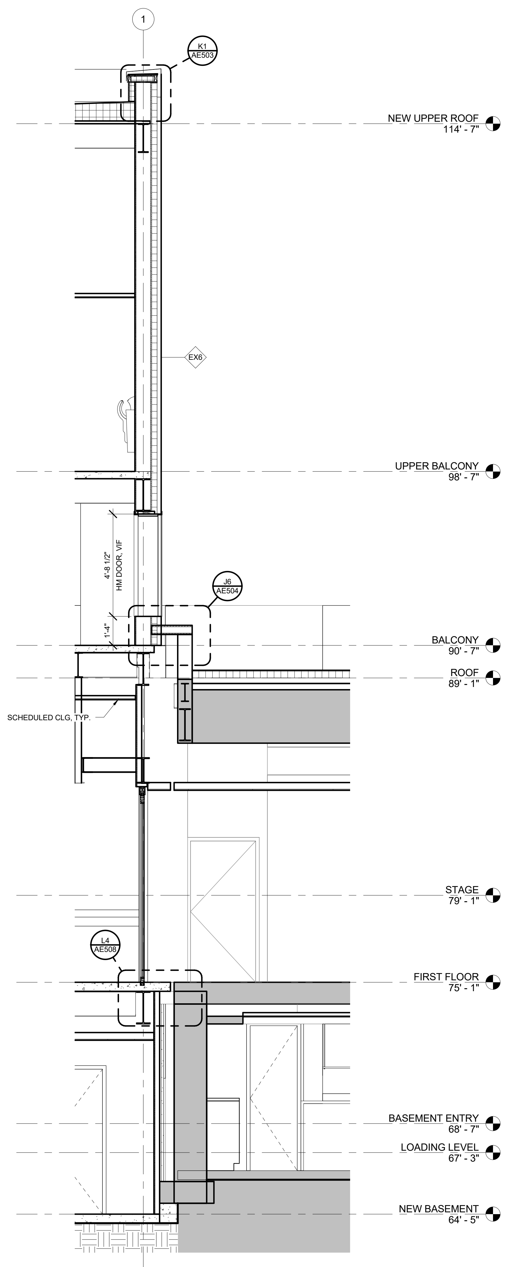
A6 WALL SECTION @ SERVICE CORRIDOR DOOR 3/8" = 1'-0" AE101B
