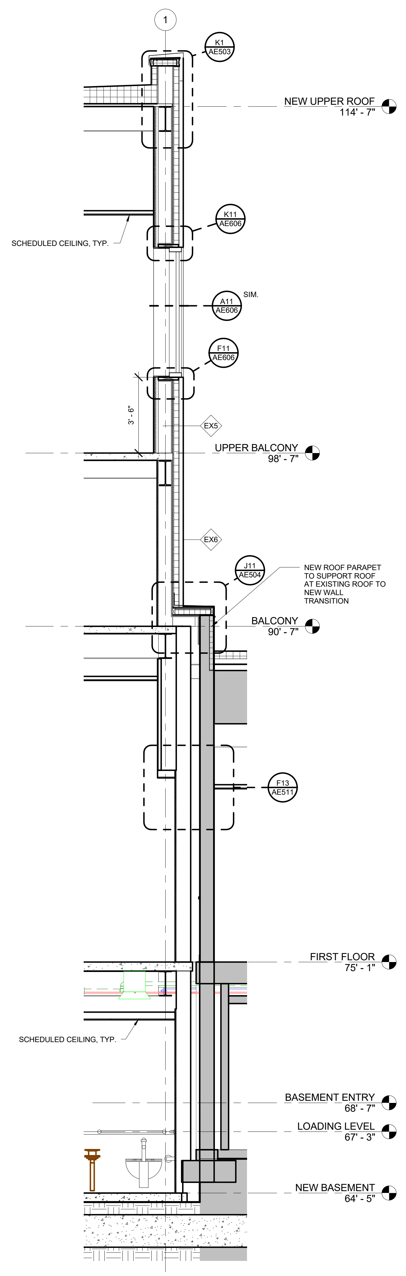
A10 WALL SECTION @ PARTI WALL 3/8" = 1'-0" AE101
