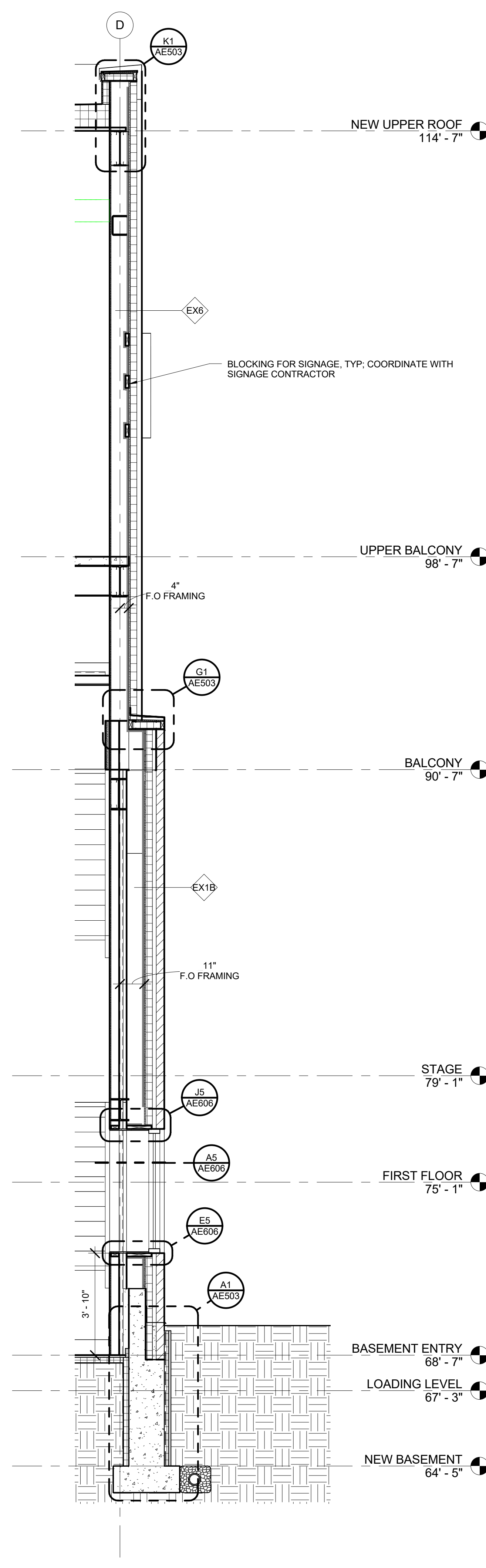
A4 WALL SECTION @ CORNER STAIR 3/8" = 1'-0" AE101
