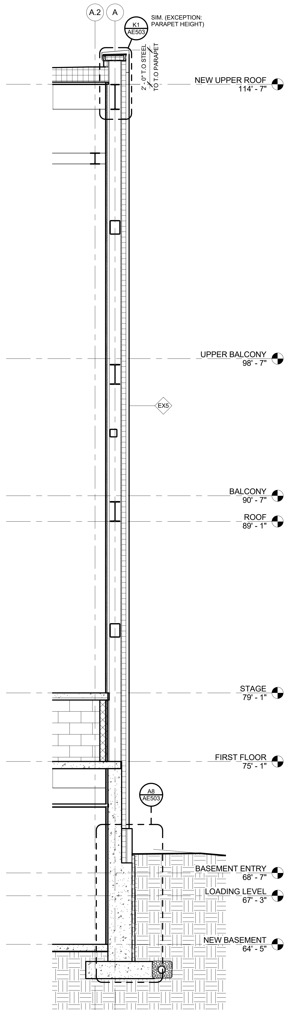
A1 WALL SECTION @ VERT. METAL PANEL 3/8" = 1'-0" AE101
