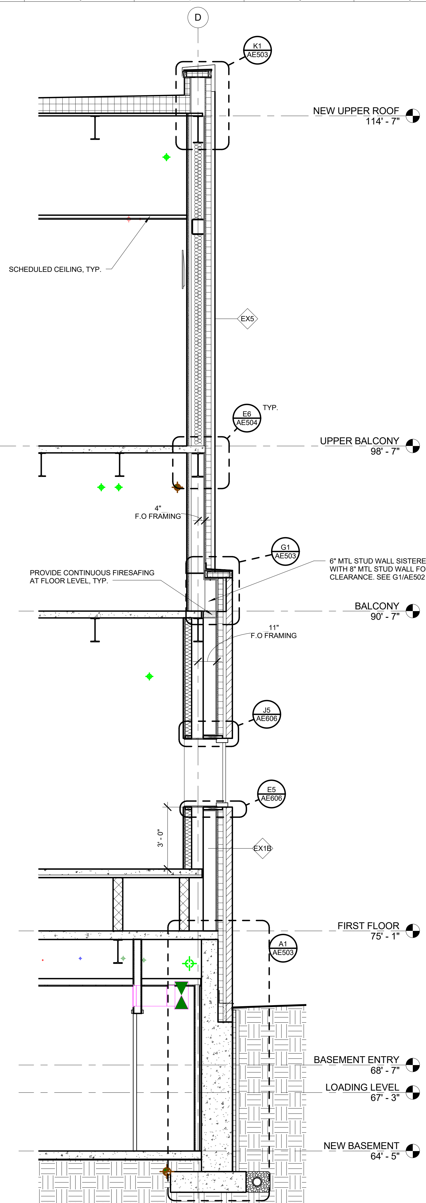
A5 TYPICAL BRICK VENEER WALL SECTION 3/8" = 1'-0" AE101
