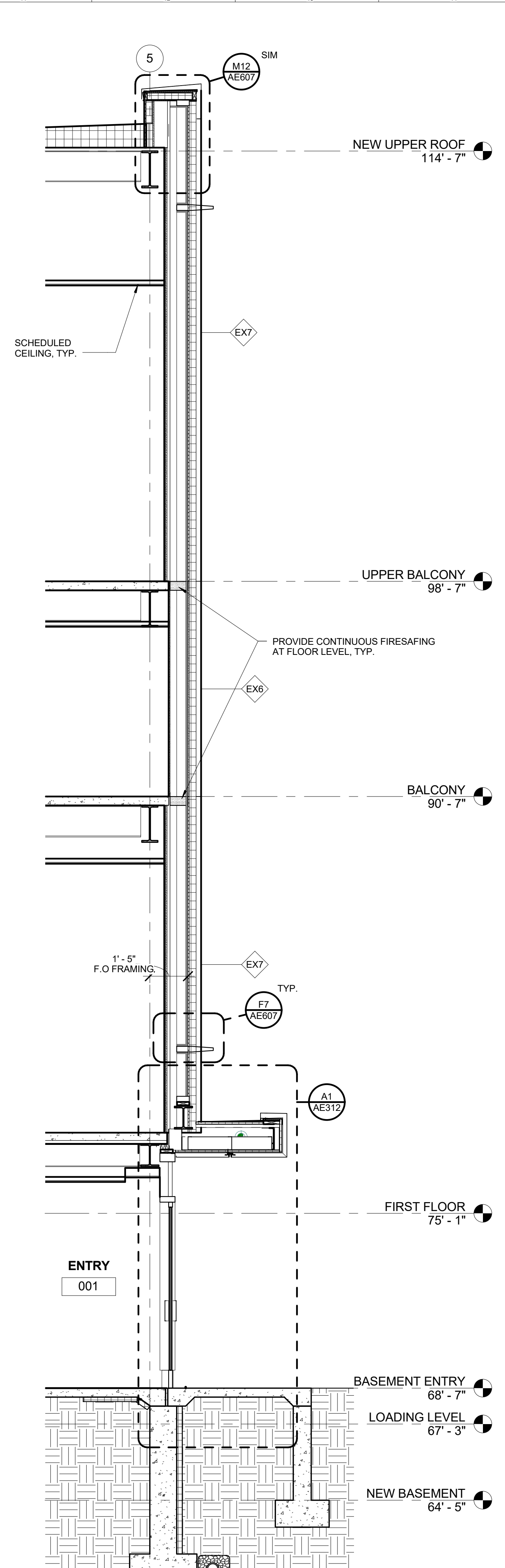
A11 TYPICAL METAL PANEL WALL SECTION 3/8" = 1'-0" AE101
