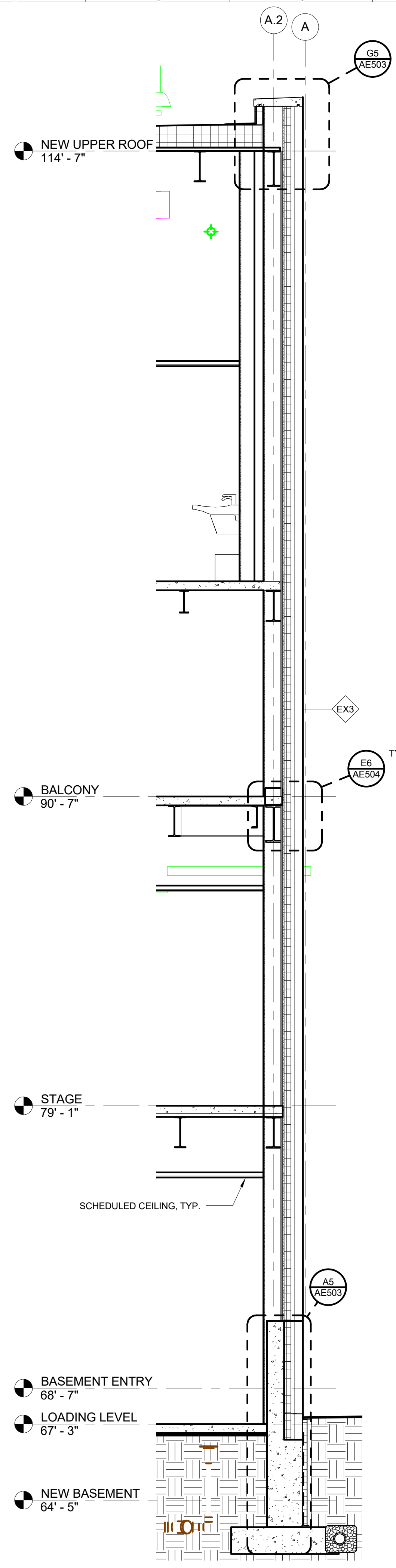
A1 TYPICAL STONE PANEL WALL SECTION 3/8" = 1'-0" AE101
