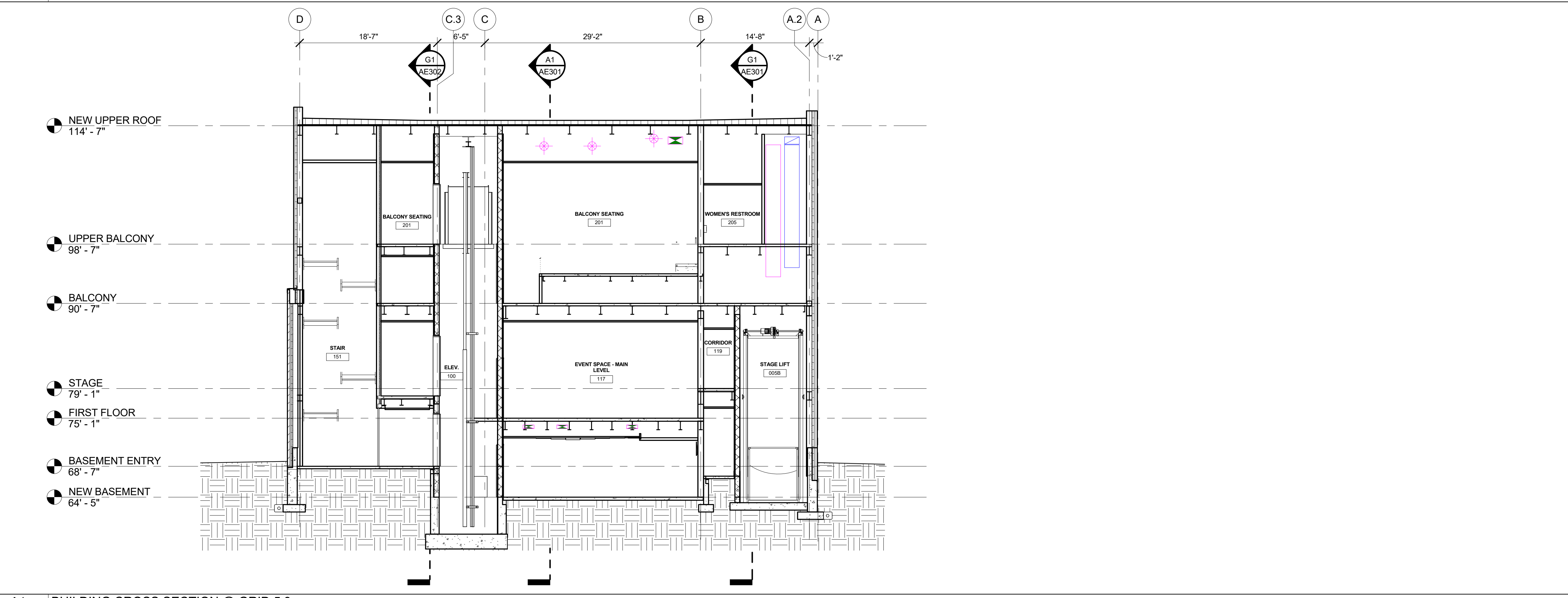
A1 BUILDING CROSS SECTION @ GRID 5.3 1/8" = 1'-0"
