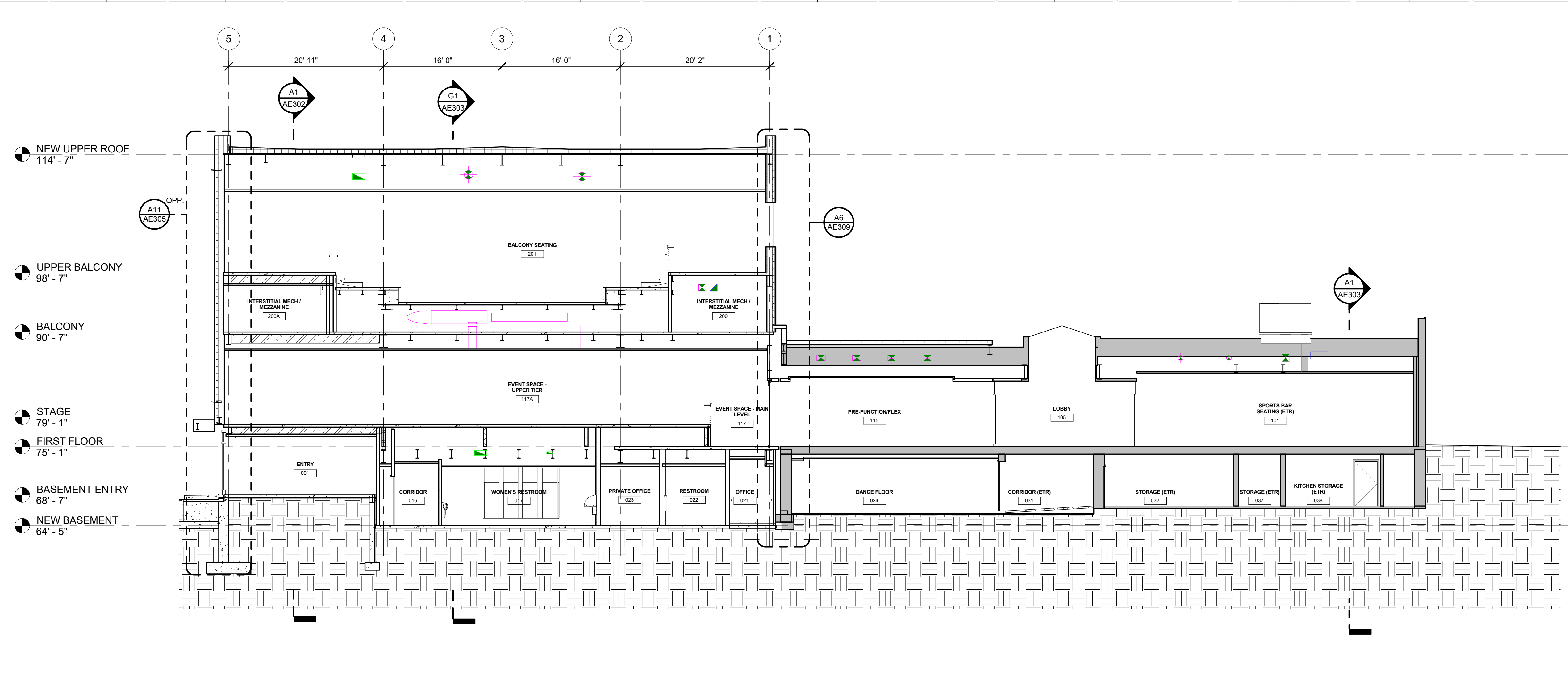
G1 BUILDING SECTION @ GRID D.5 1/8" = 1'-0"
