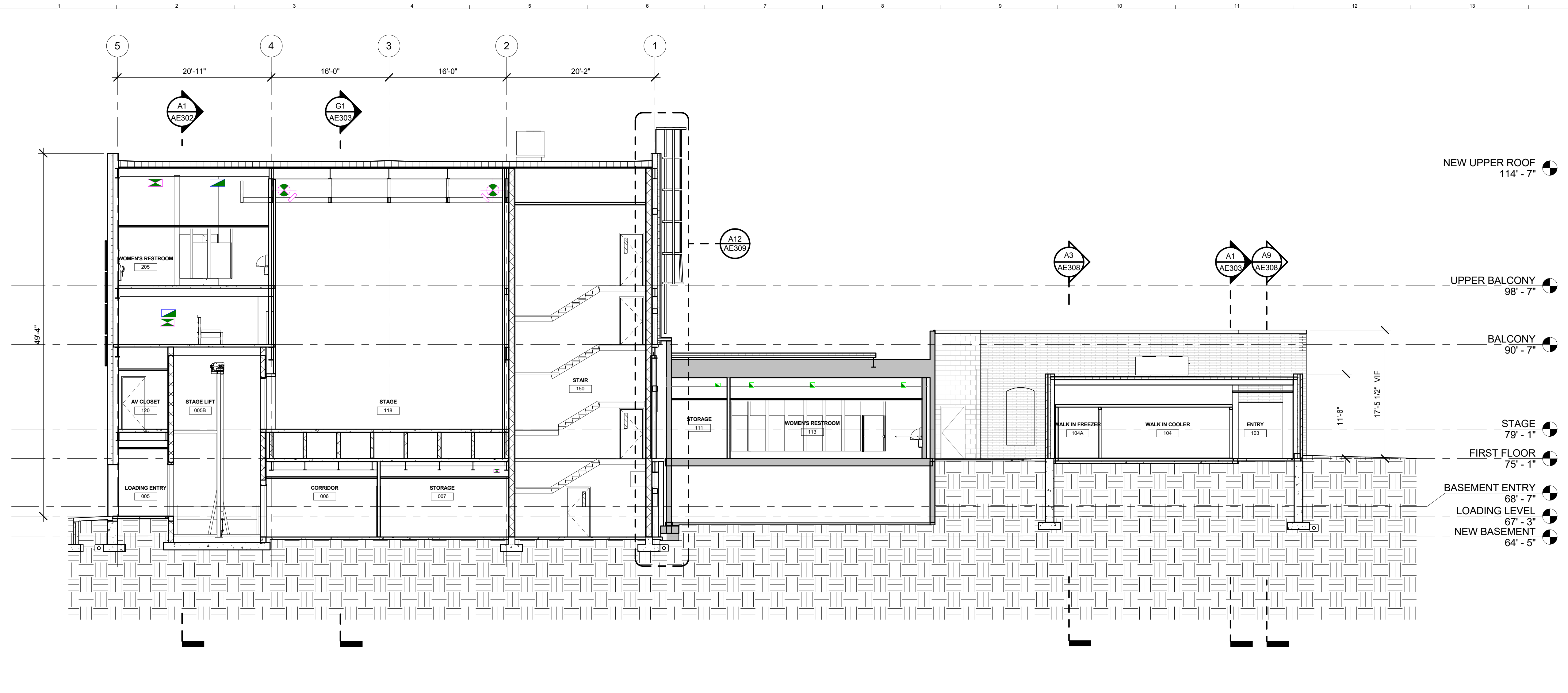
G1 BUILDING SECTION @ GRID A.5 1/8" = 1'-0"
