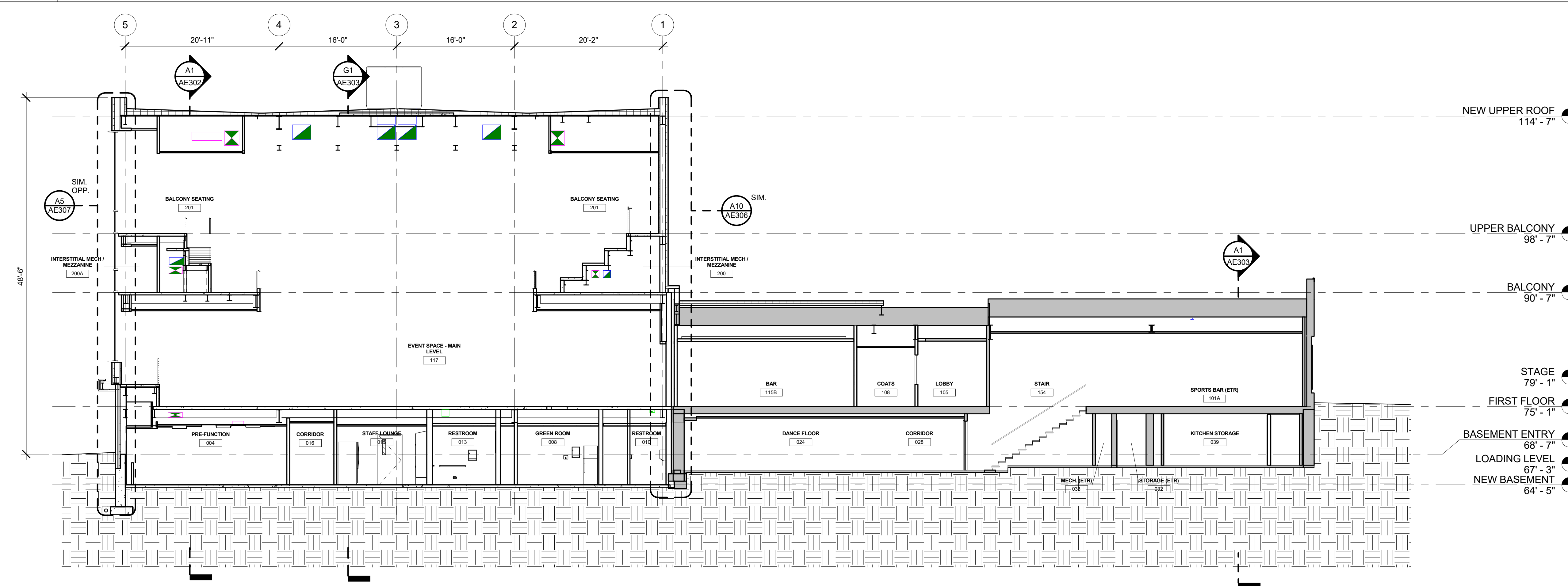
A1 BUILDING SECTION @ GRID C.9 1/8" = 1'-0"
