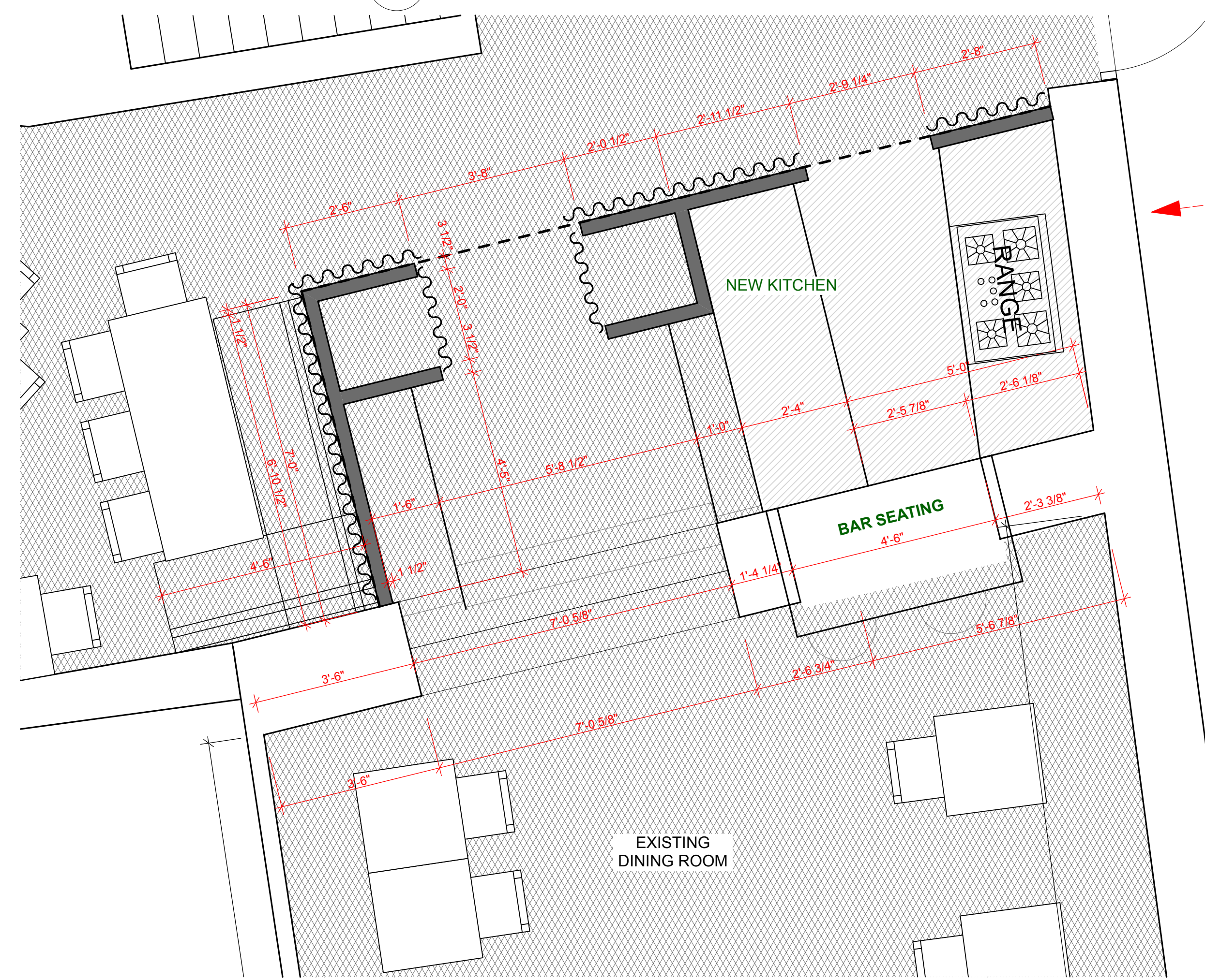
3 NEW KITCHEN SCALE: 1/2" = 1'-0"
