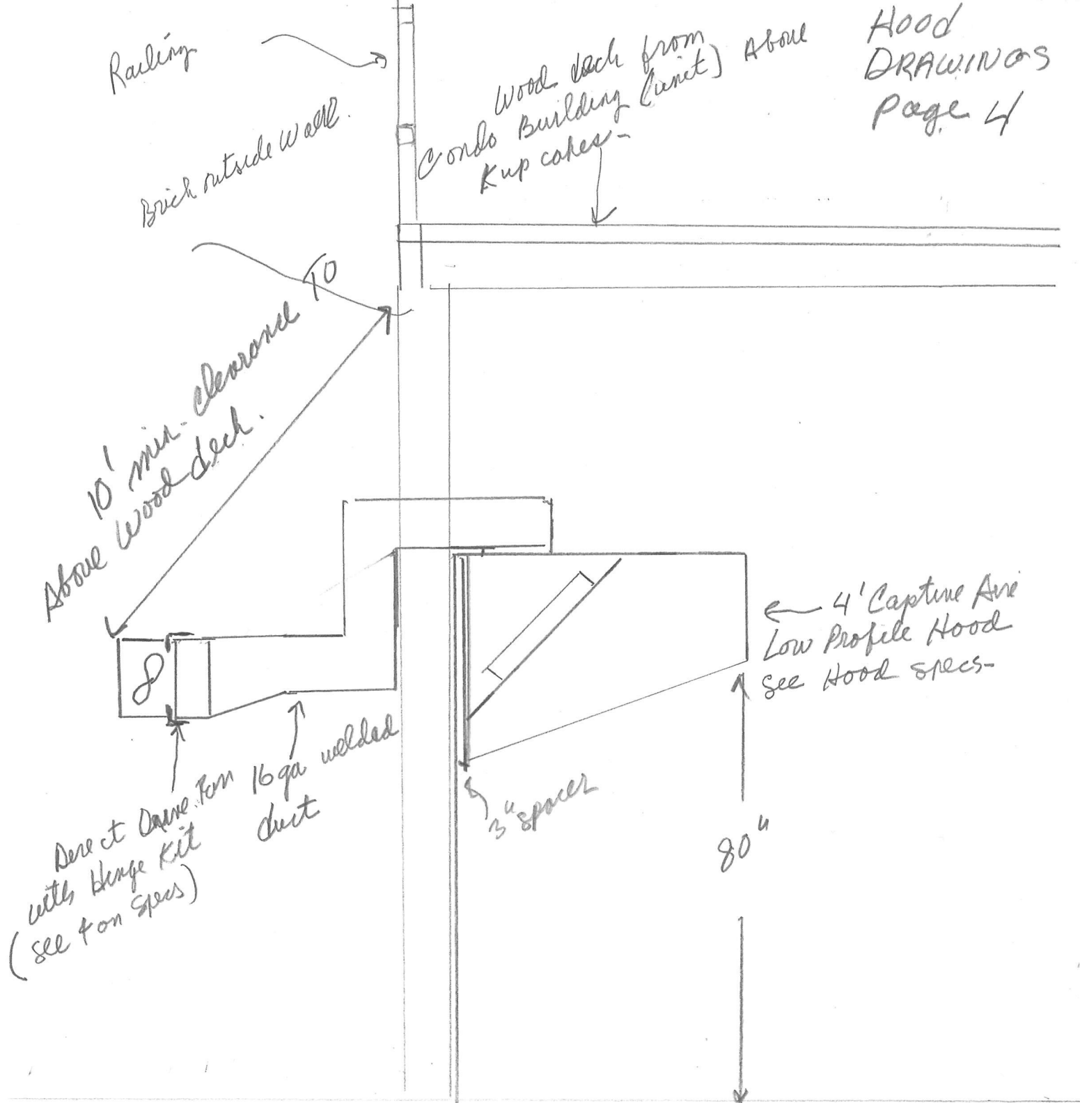
SIDE VIEW
