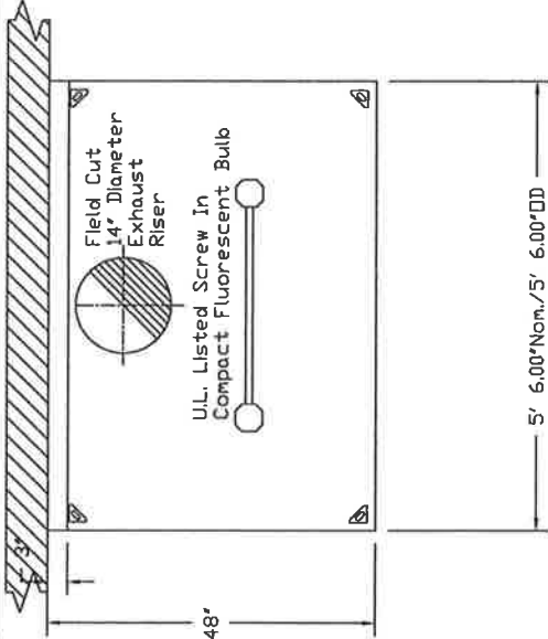
PLAN VIEW - Hood #1 5' 6.00" LONG 4812SND-2
