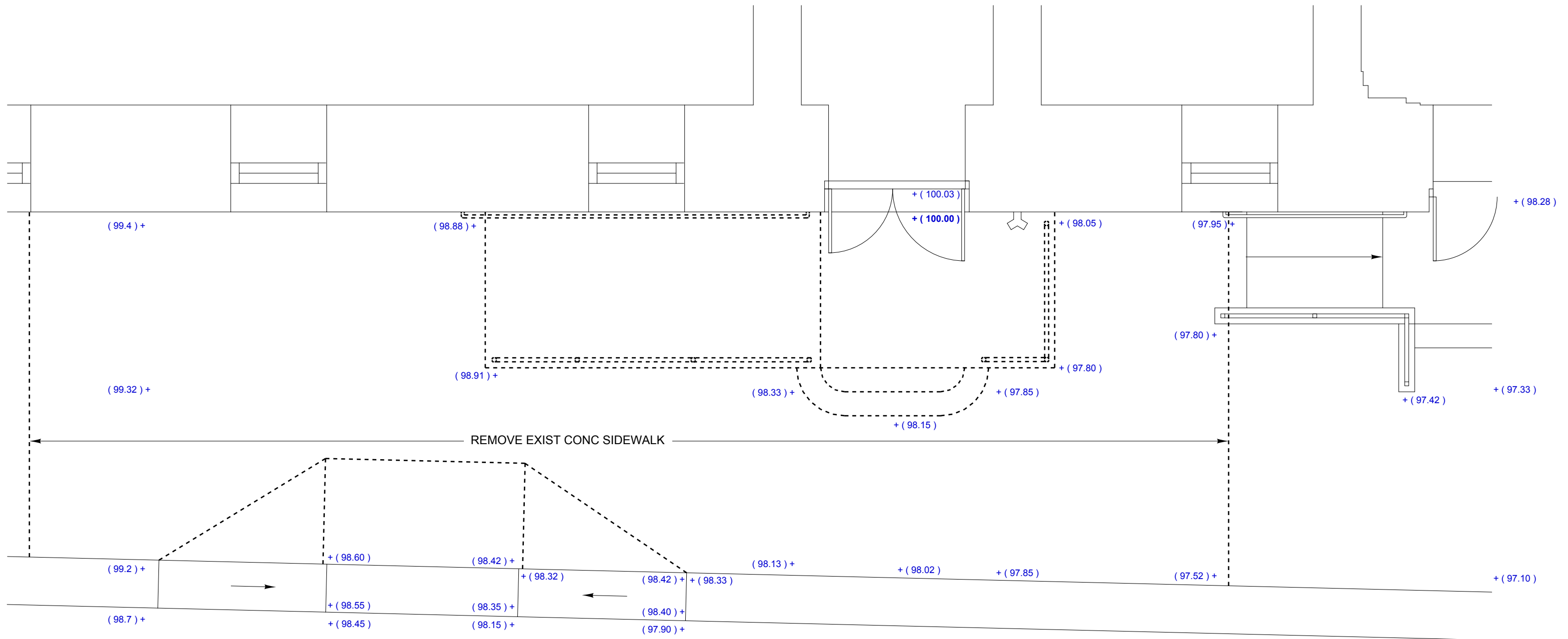
Entrance Demolition Plan 1/4"=1'-0"
