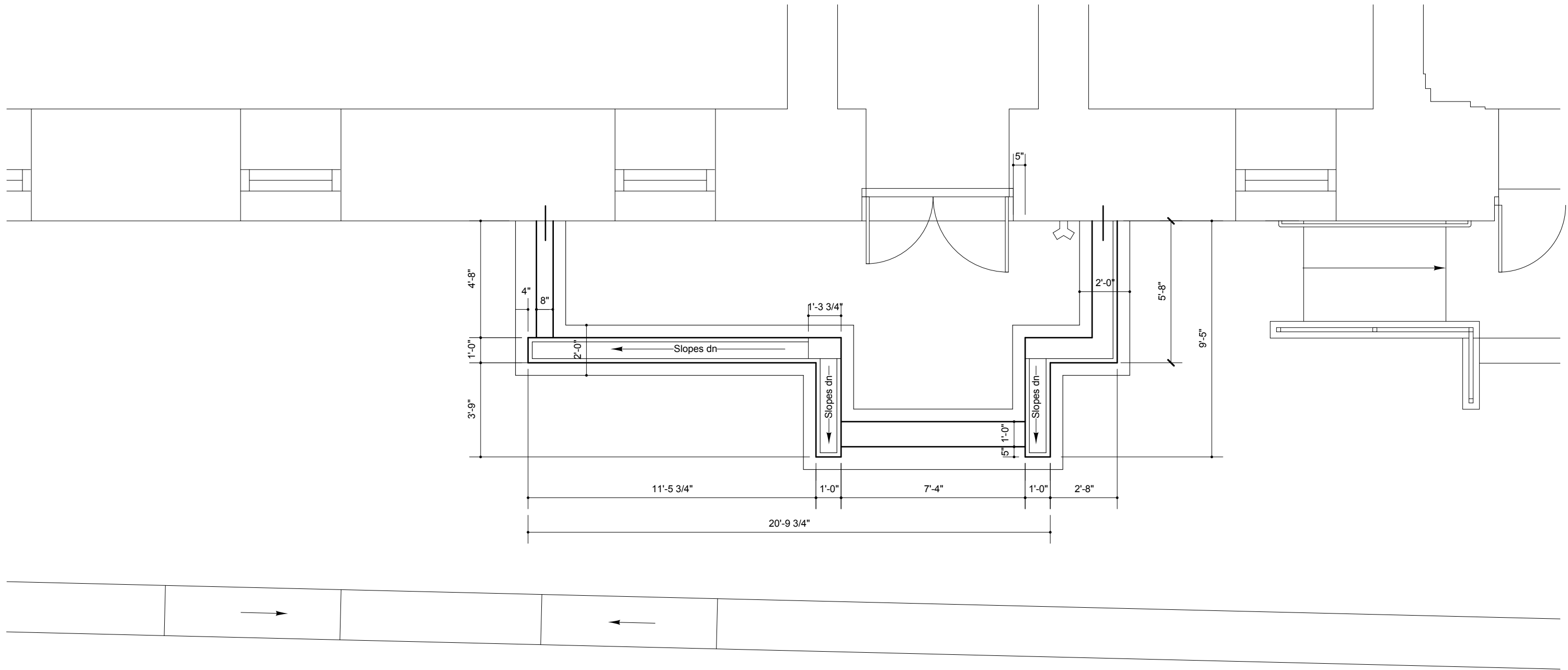
Entrance Foundation Plan 1/4"=1'-0"
