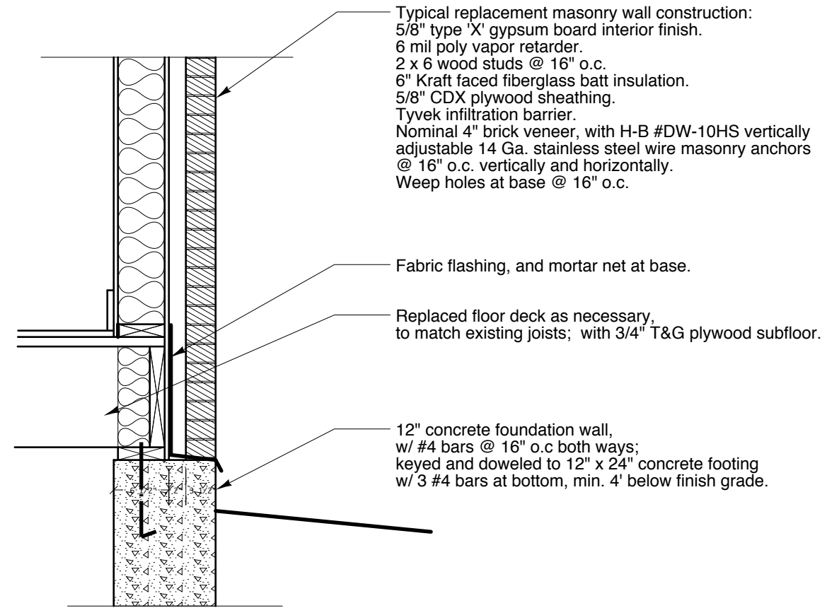
Section Through New Stair Wall (where gymnasium removed) Scale: 3/4" = 1'-0"
