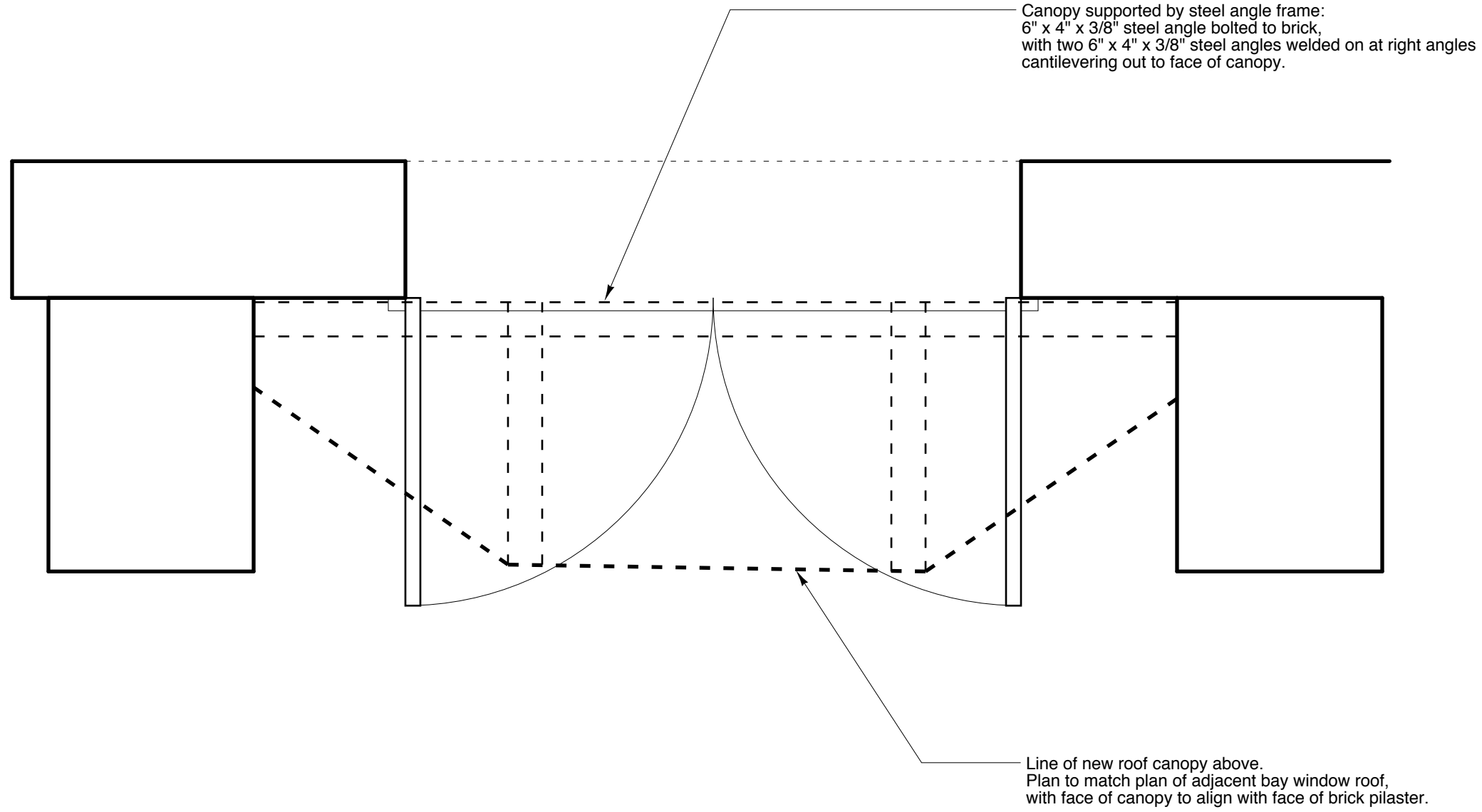
Plan of New Canopy Roof at Function Room Entrance (see SK3 for elevation and section)
