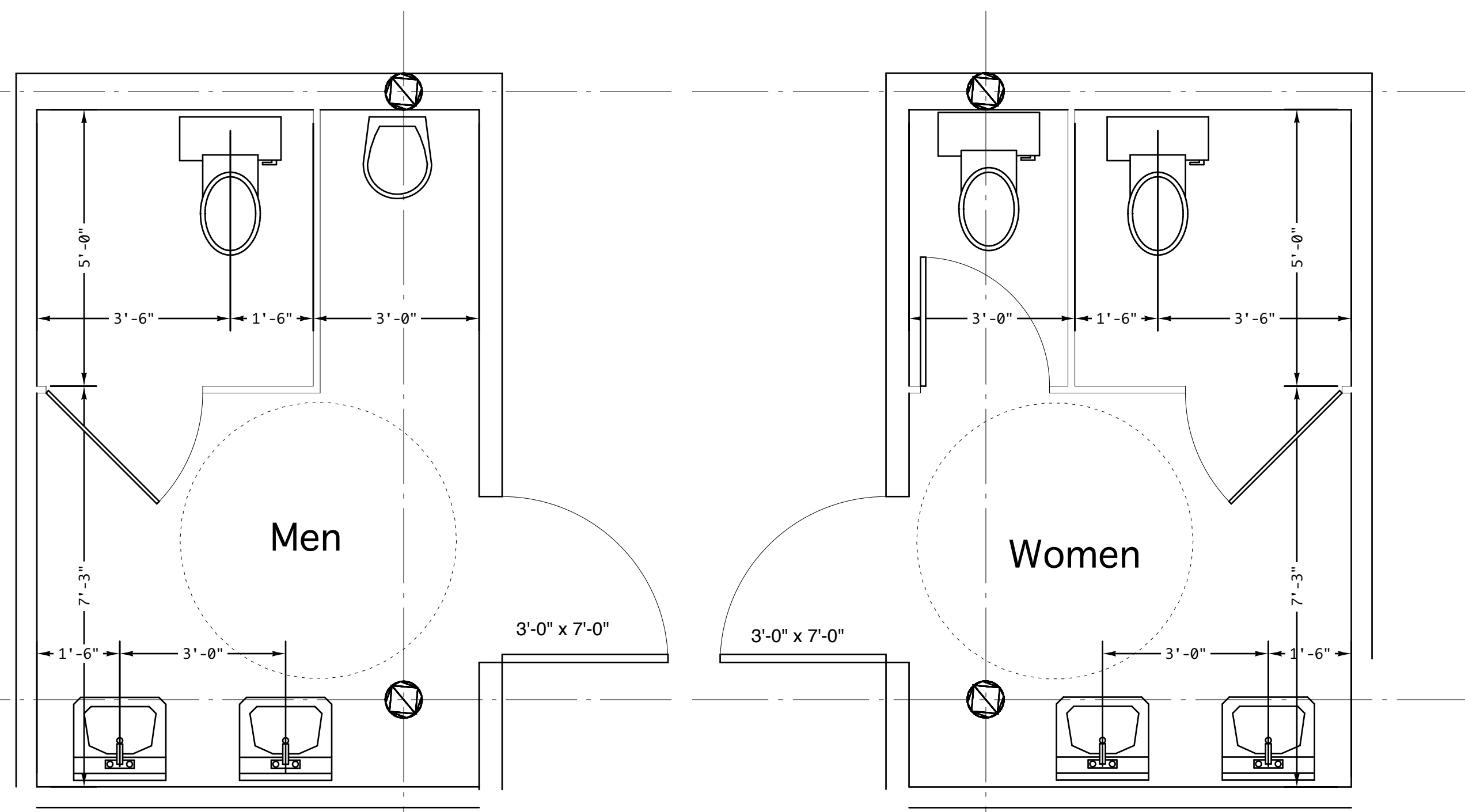
First Floor Men's & Women's HCP Bathrooms Scale: 1/2" = 1'-0"
