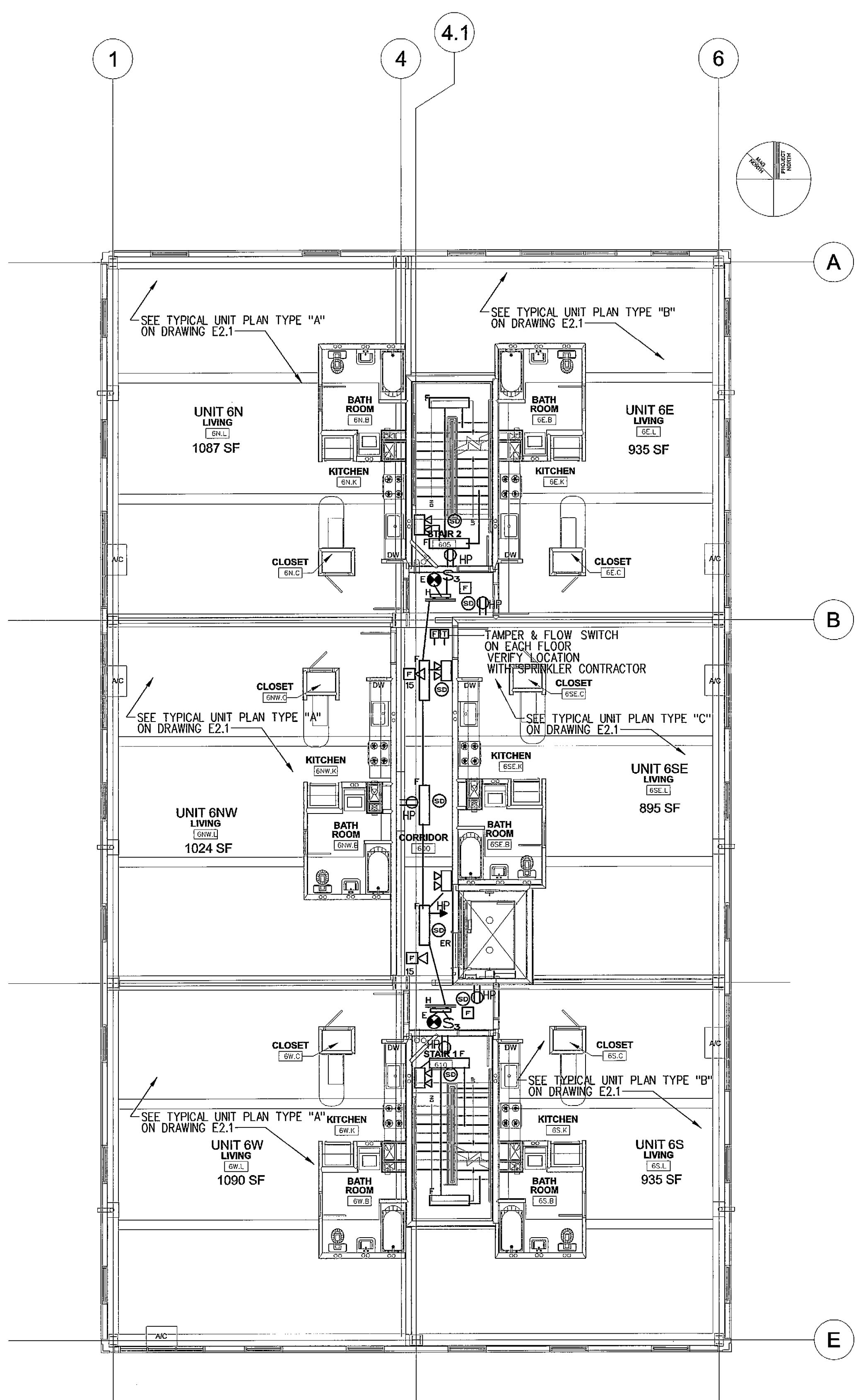
TYPICAL 2ND - 4TH & 6TH FLOOR ELECTRICAL PLAN SCALE: 1/8"=1'-0"
