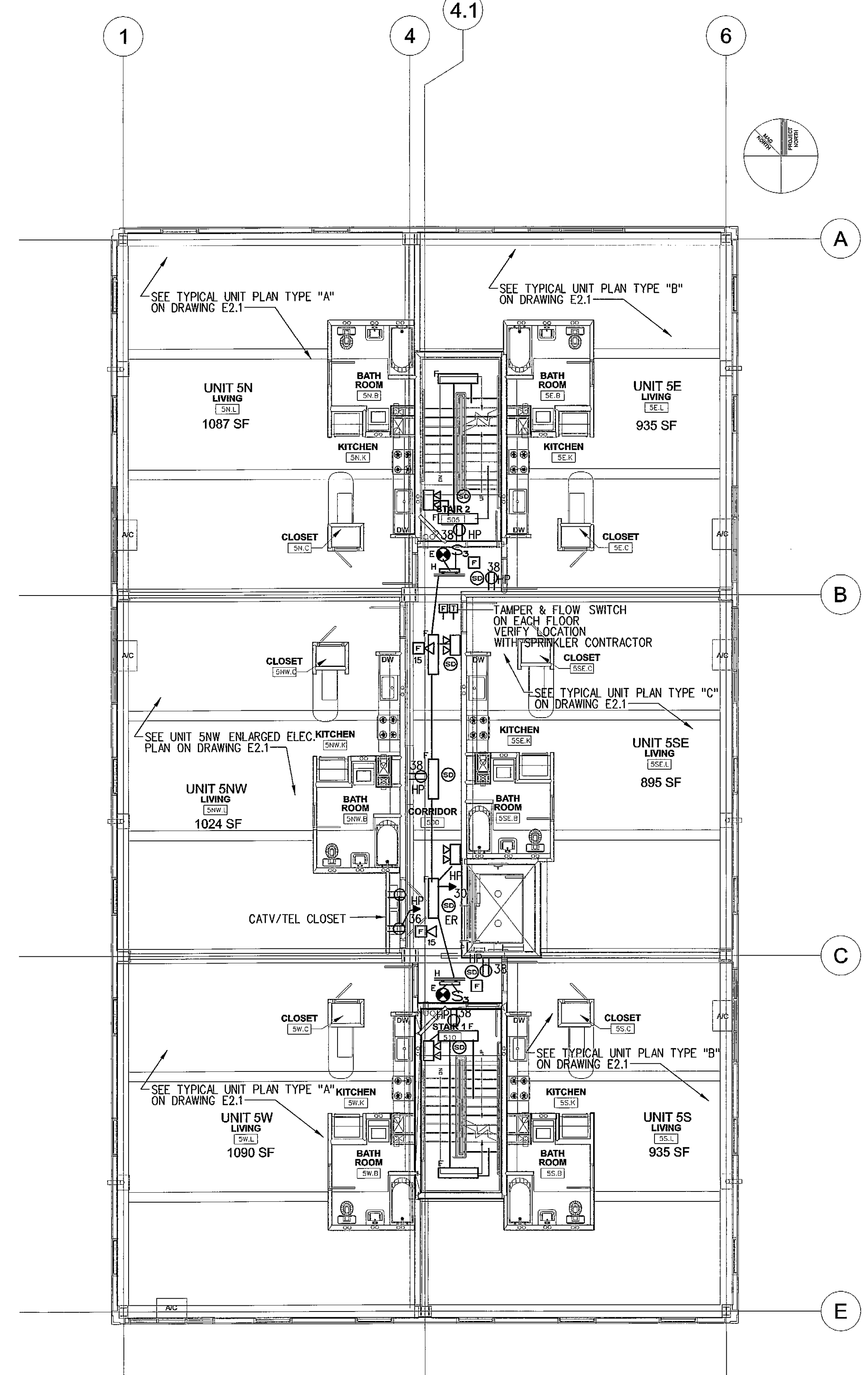
FIFTH FLOOR ELECTRICAL PLAN SCALE: 1/8"=1'-0"
