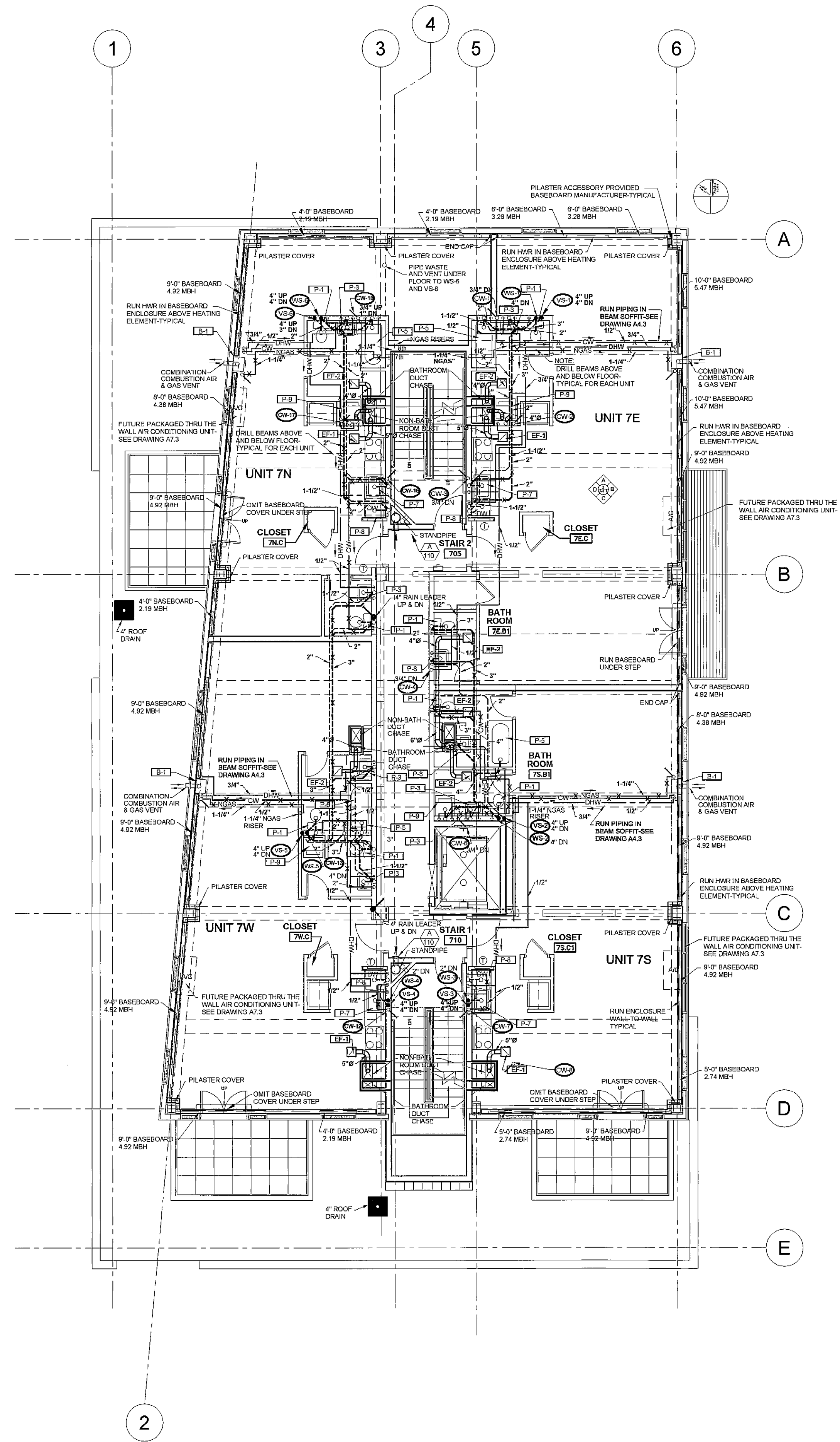
1 SEVENTH FLOOR MECHANICAL PLAN A1.4 1/8" = 1'-0"
