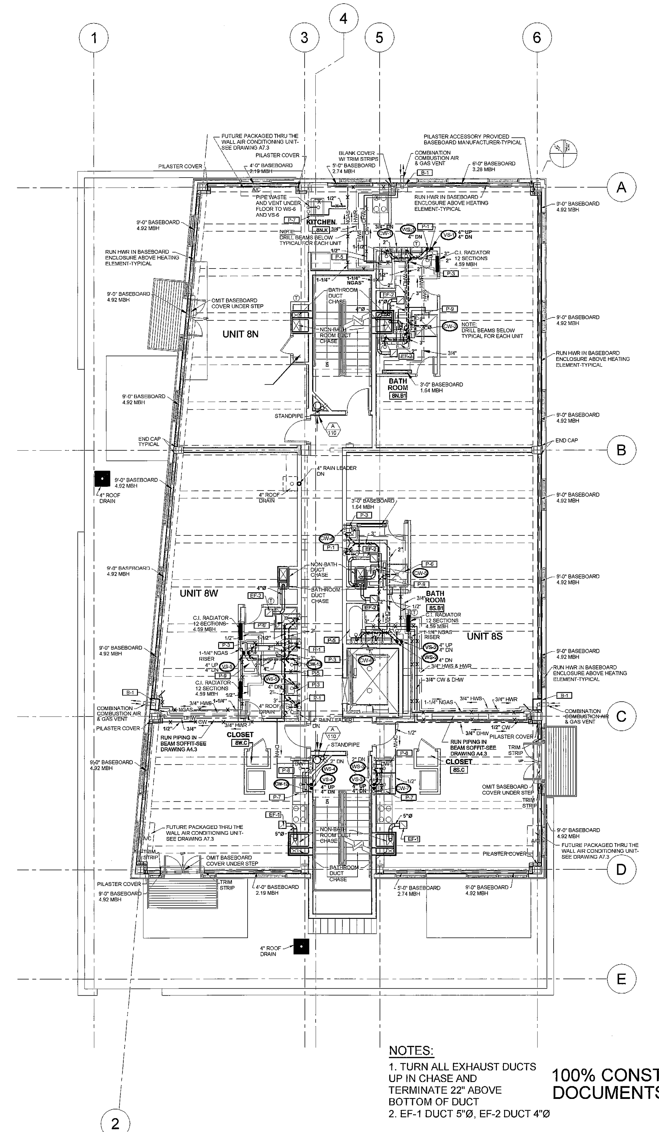
2 EIGHTH FLOOR MECHANICAL PLAN A1.4 1/8" = 1'-0"
