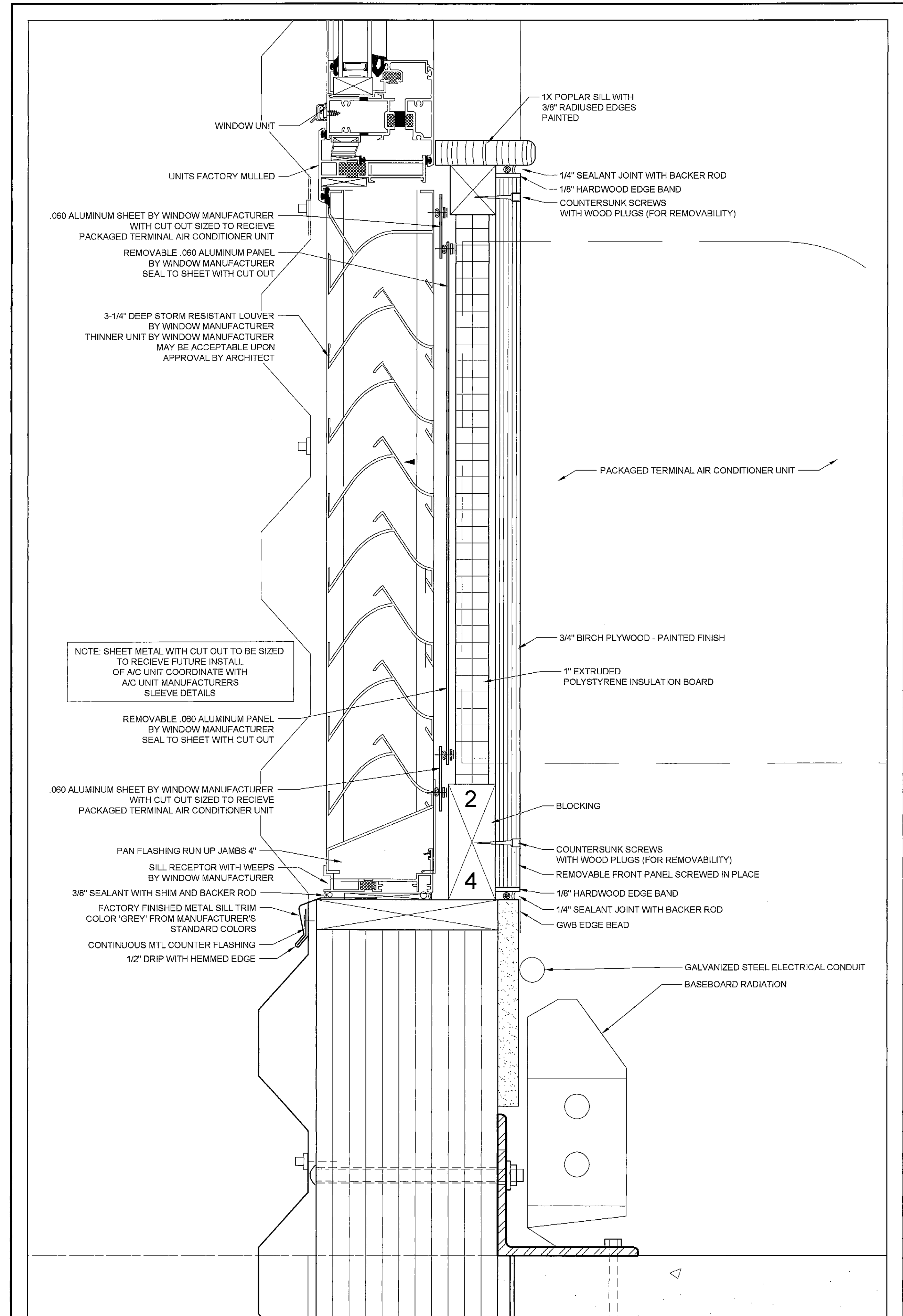
1 LOUVER SECTION DETAIL AT WINDOW WALL A7.3 8" = 1'-0"
