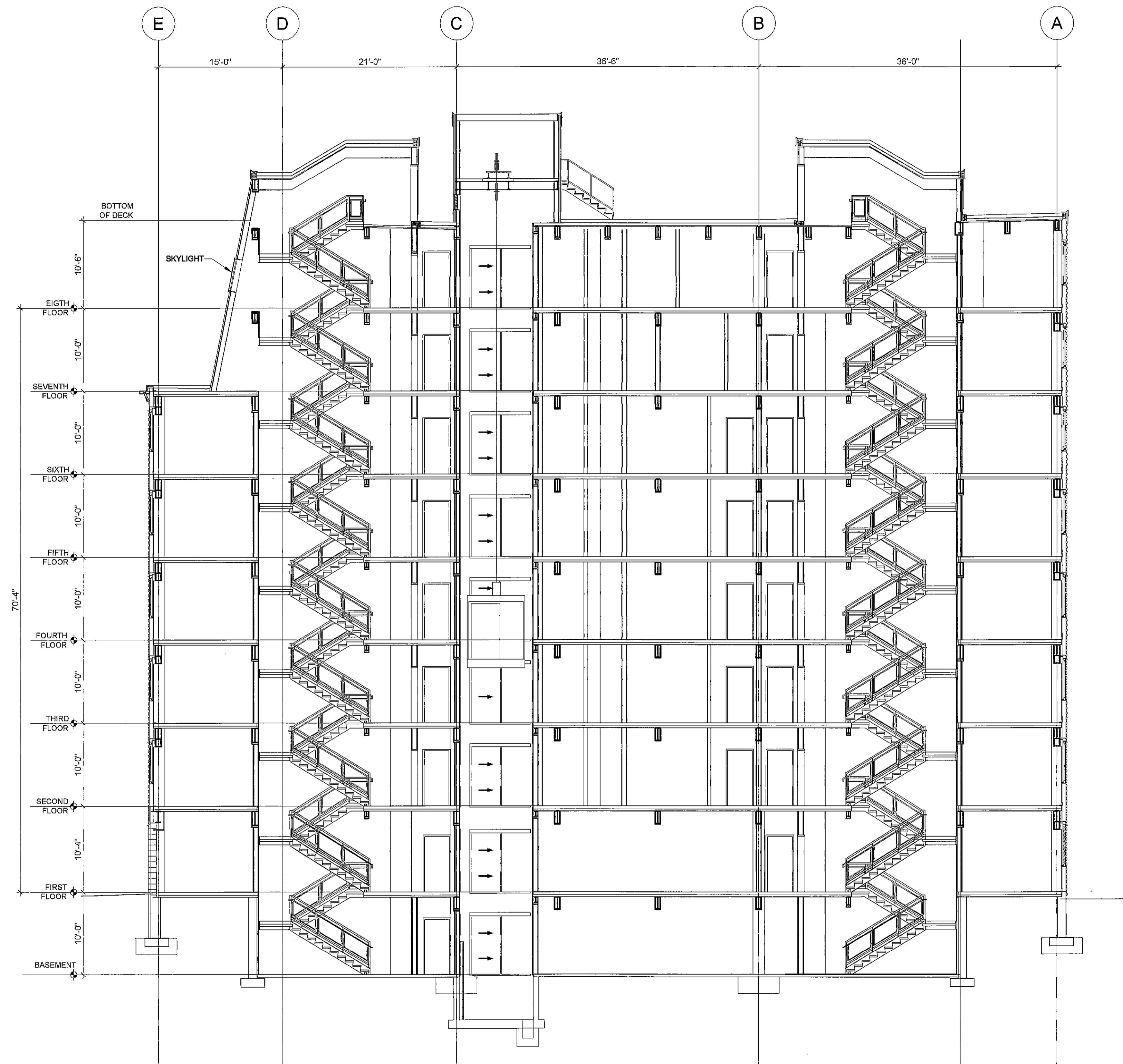
2 BUILDING LONGITUDINAL SECTION 1/8" = 1'-0"
