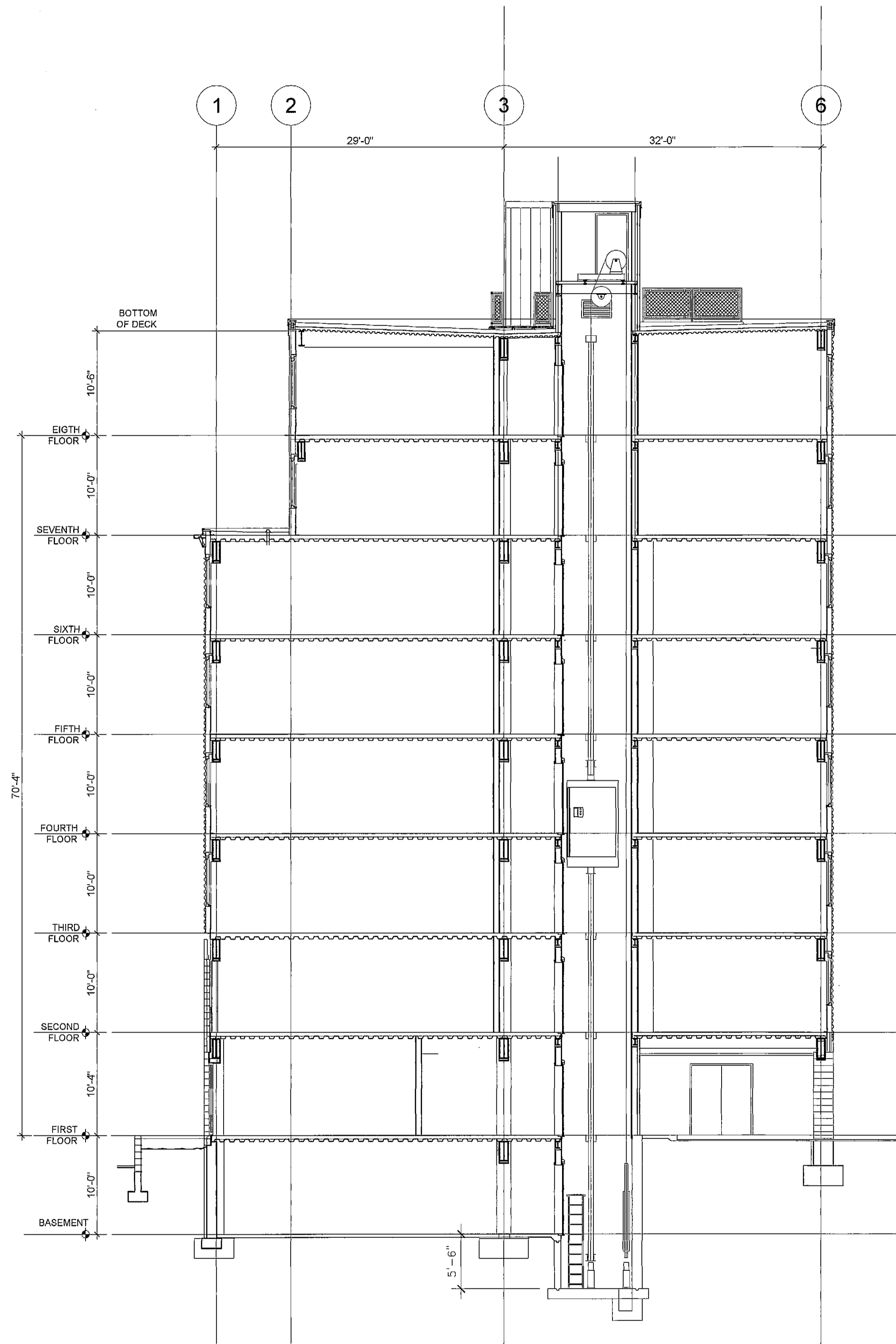
1 BUILDING CROSS SECTION 1/8" = 1'-0"
