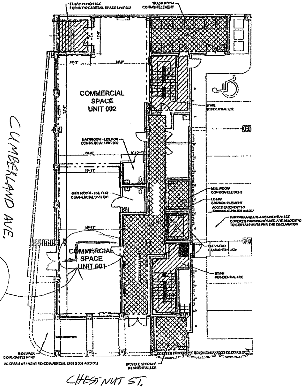
1 FIRST FLOOR PLAN
