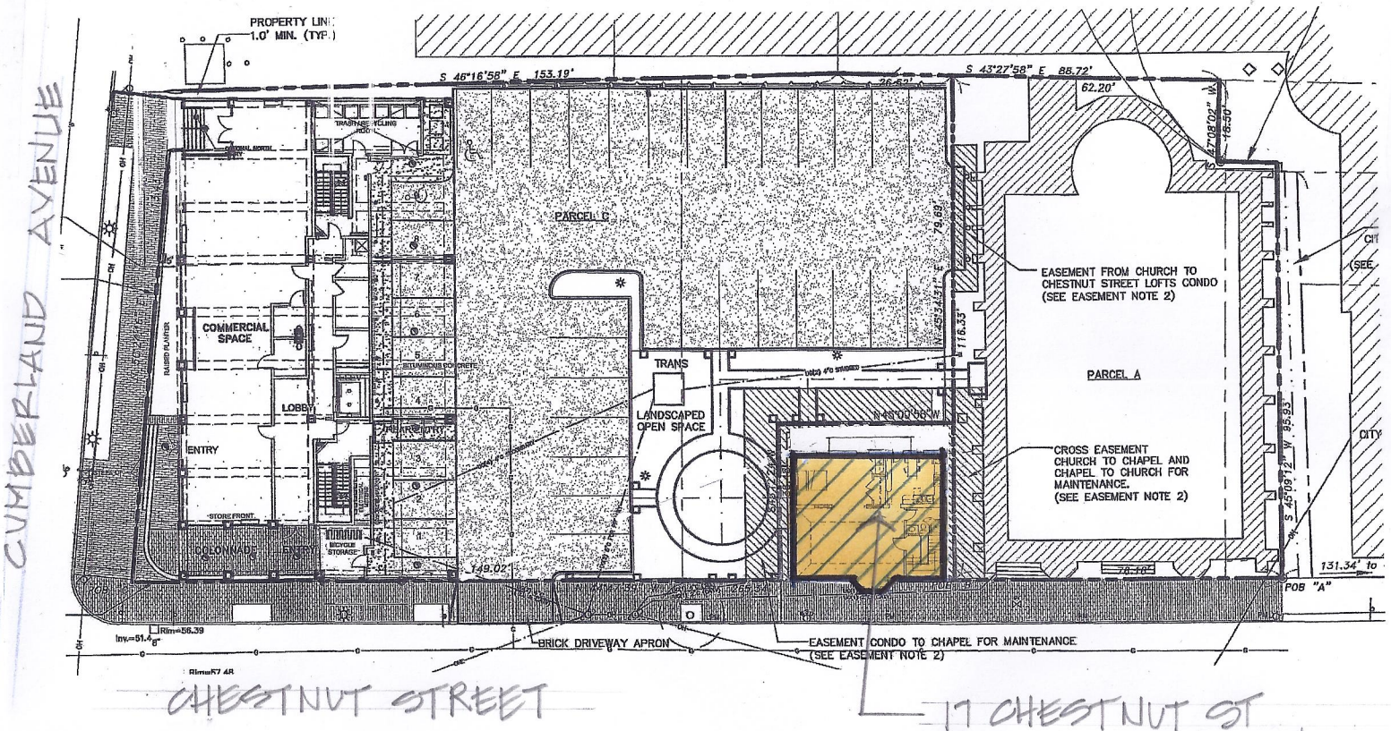
Site Plan 1" = 40'-0"
