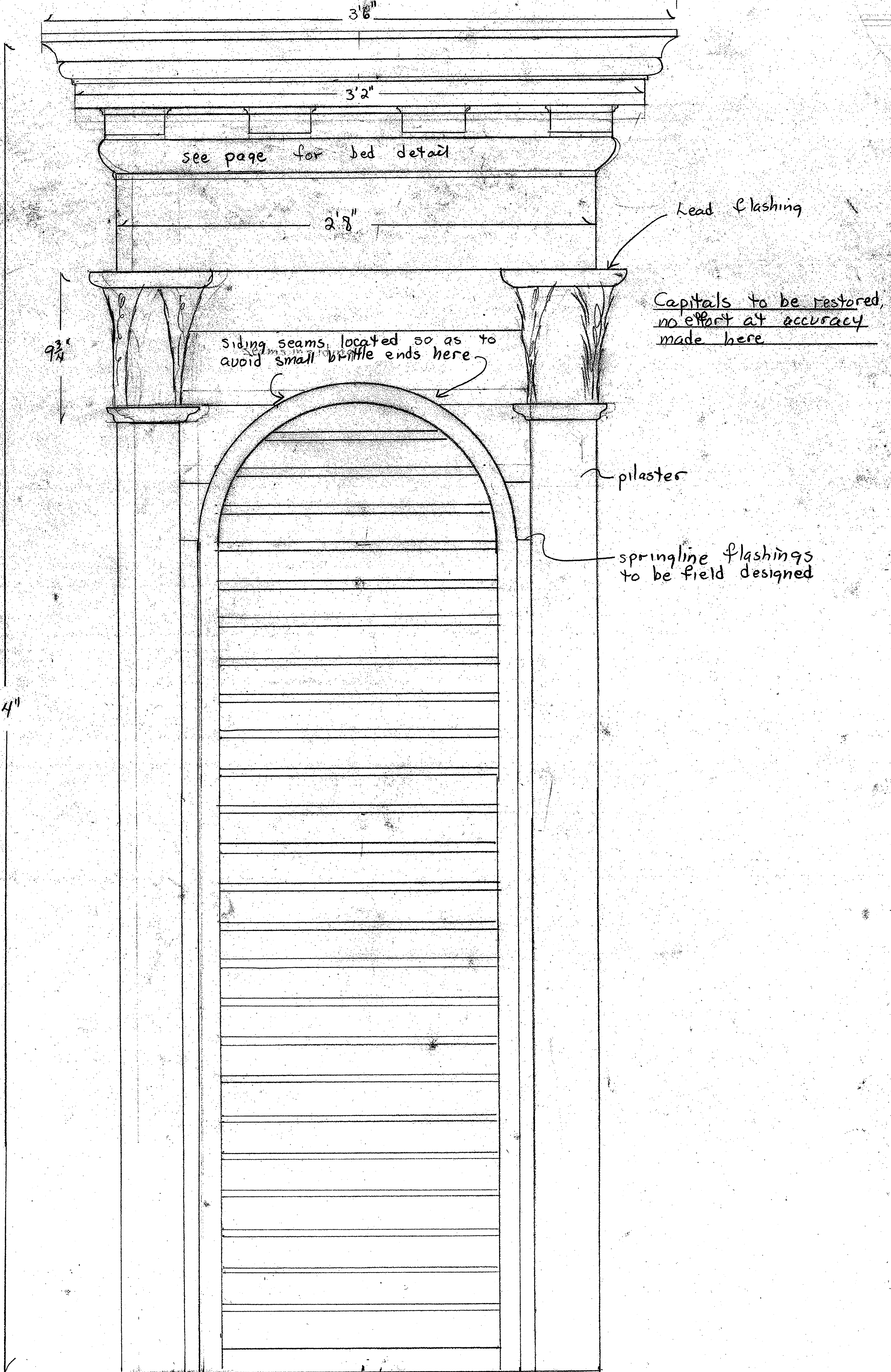
⑥ Lantern Face Elevation 3"=1'
