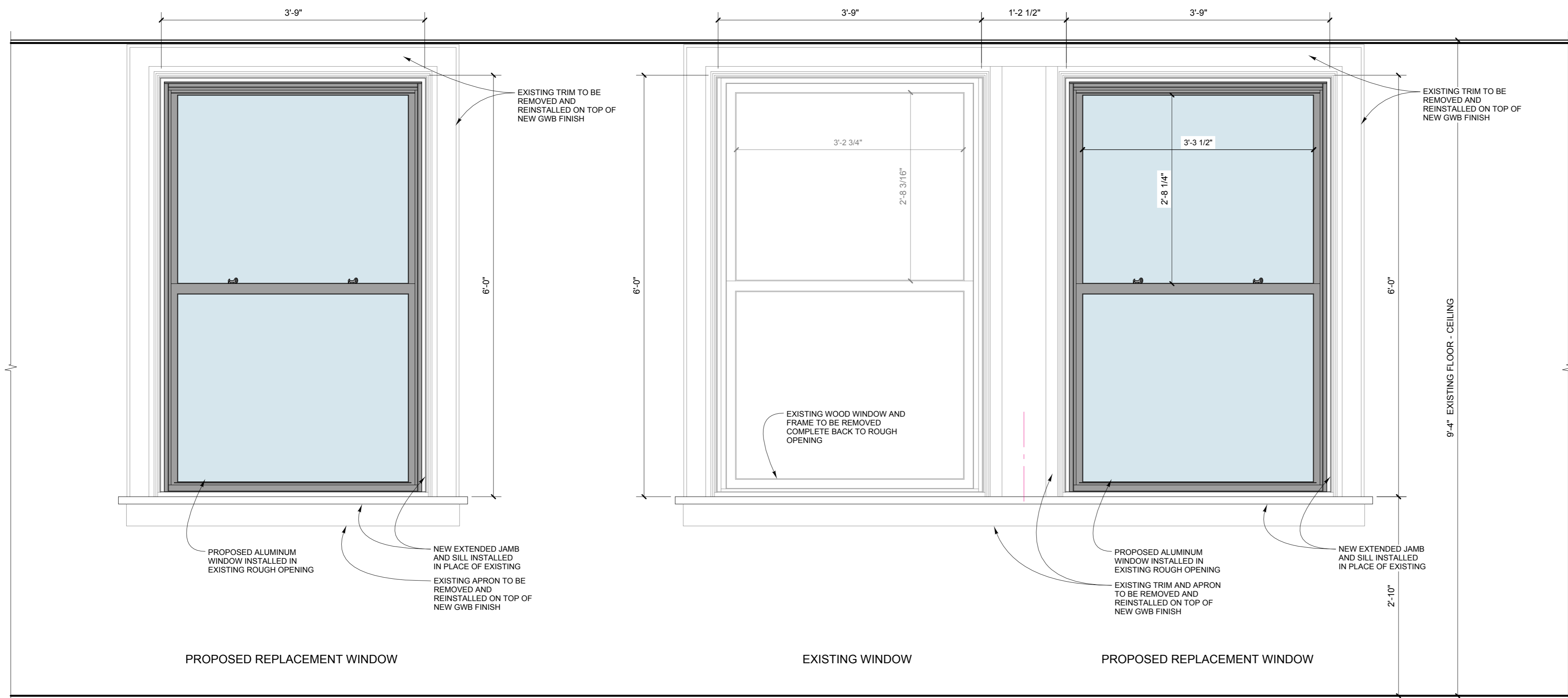
1 WINDOW ELEVATION 1" = 1'-0"
