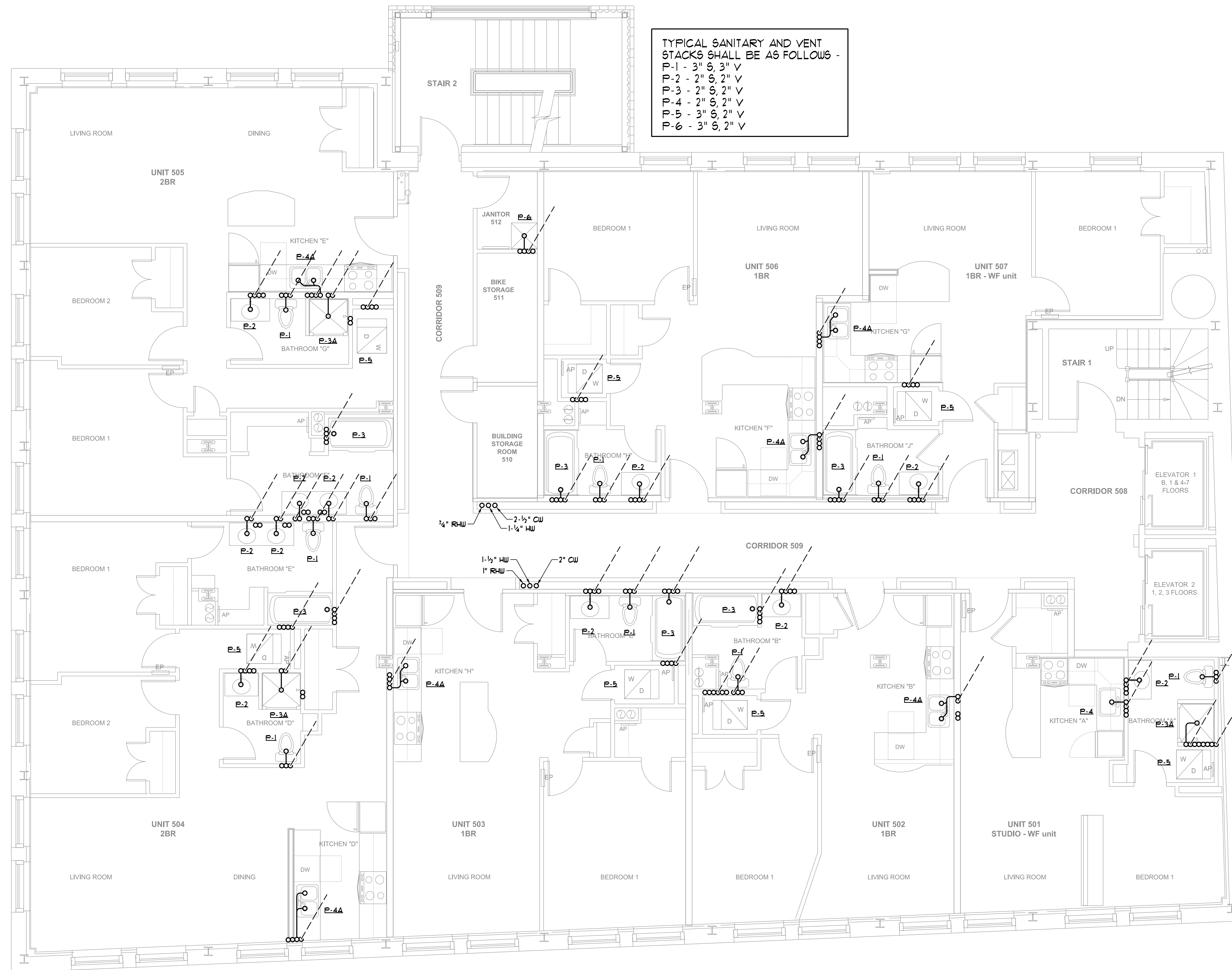
FIFTH FLOOR PLUMBING PLAN SCALE - 1/4" = 1'-0"
