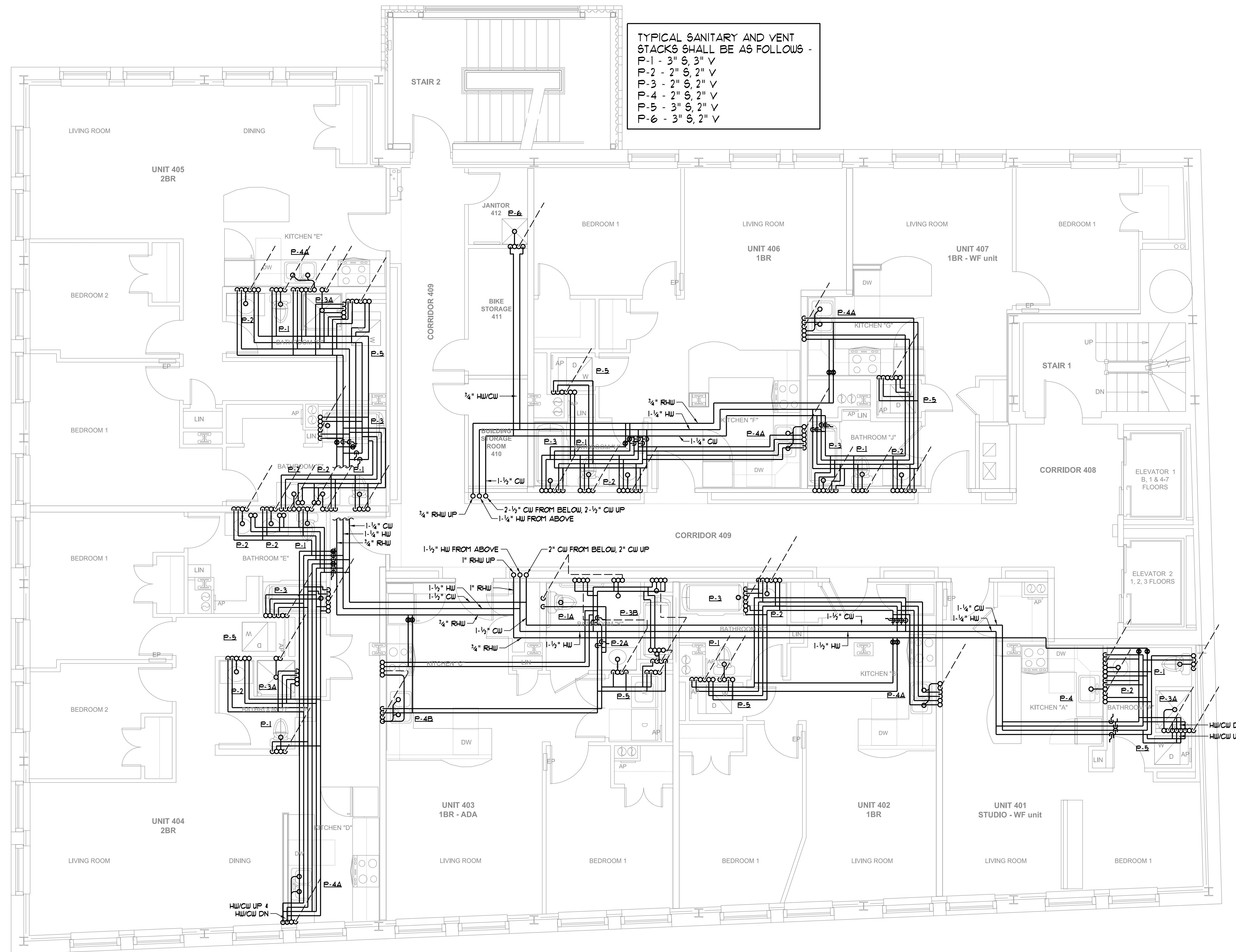
FOURTH FLOOR PLUMBING PLAN SCALE - 1/4" = 1'-0"
