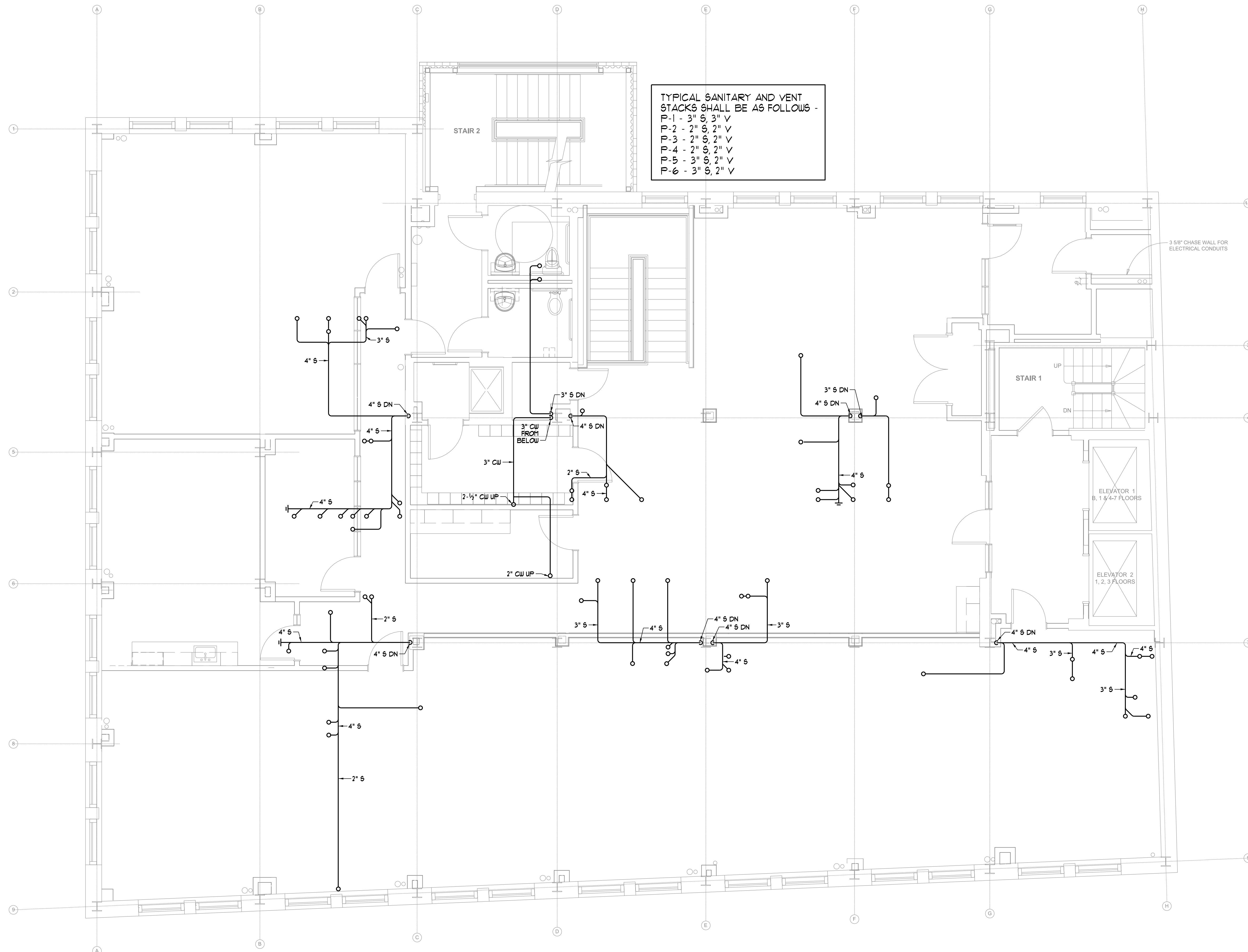
THIRD FLOOR PLUMBING PLAN SCALE - 1/4" = 1'-0"
