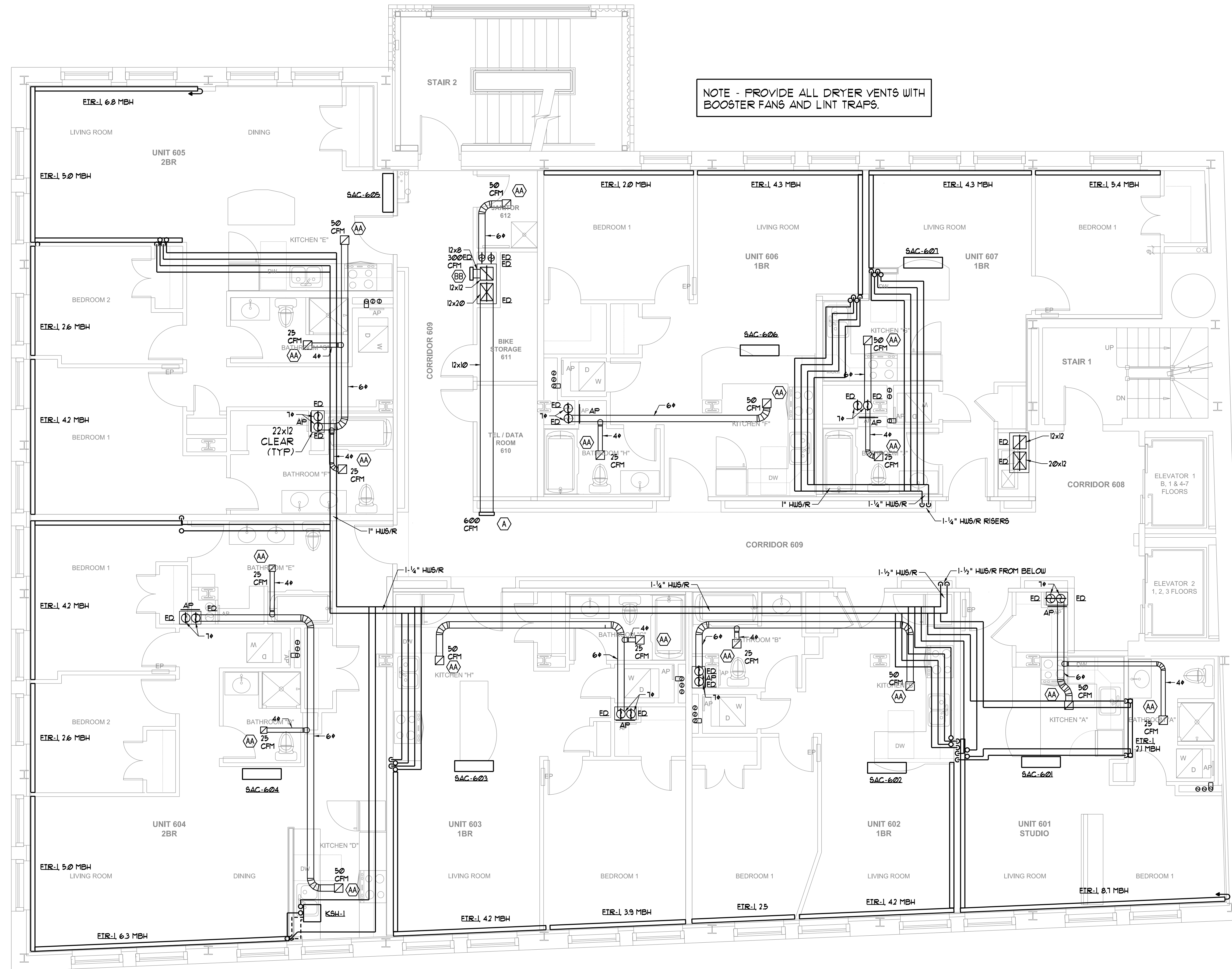
SIXTH FLOOR MECHANICAL PLAN SCALE - 1/4" = 1'-0"
