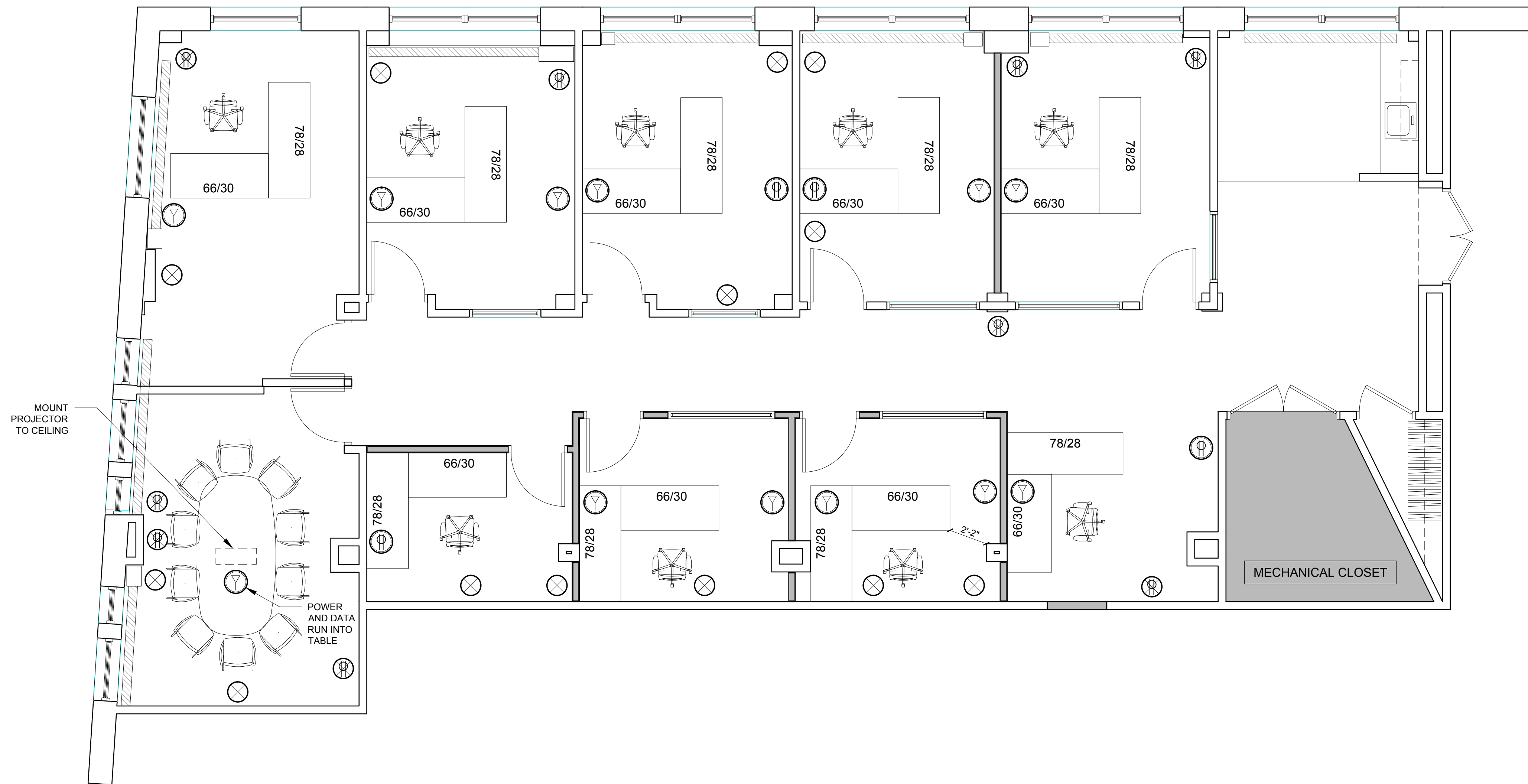
1 TELEPHONE / DATA PLAN 1/4" = 1'-0"
