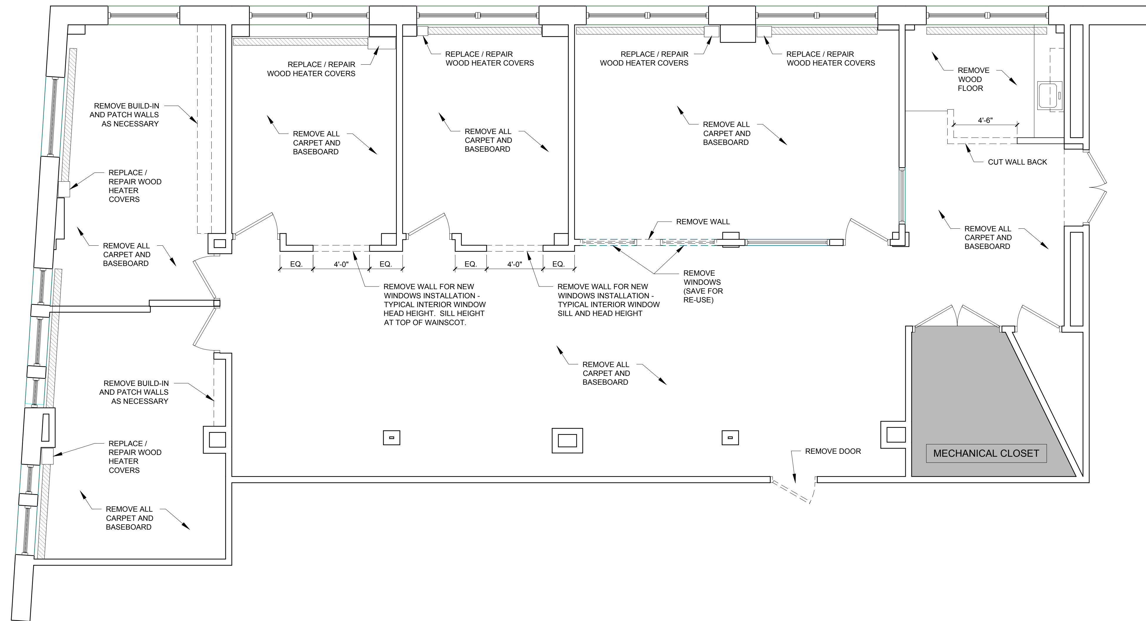
1 DEMO PLAN 1/4" = 1'-0"
