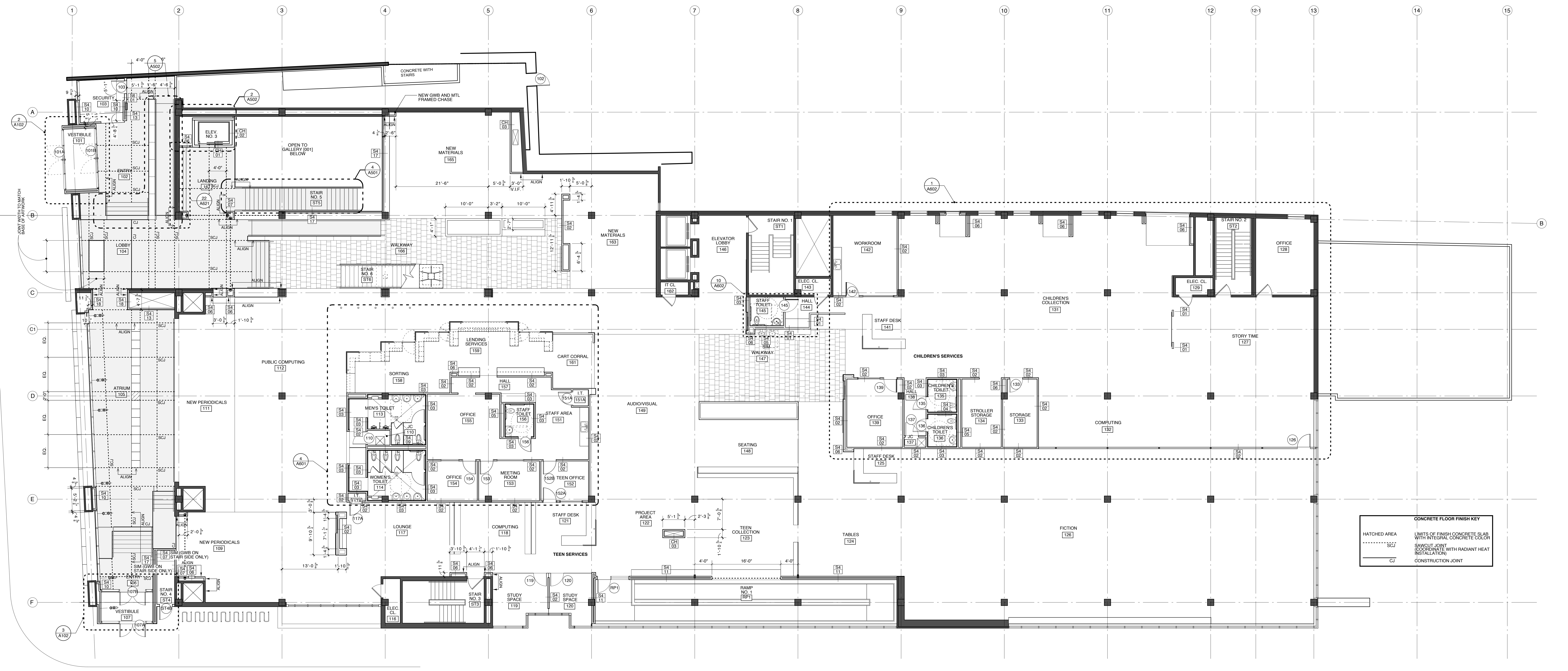
1 MAIN LEVEL DIMENSION PLAN SCALE: 1/8" = 1'-0"
