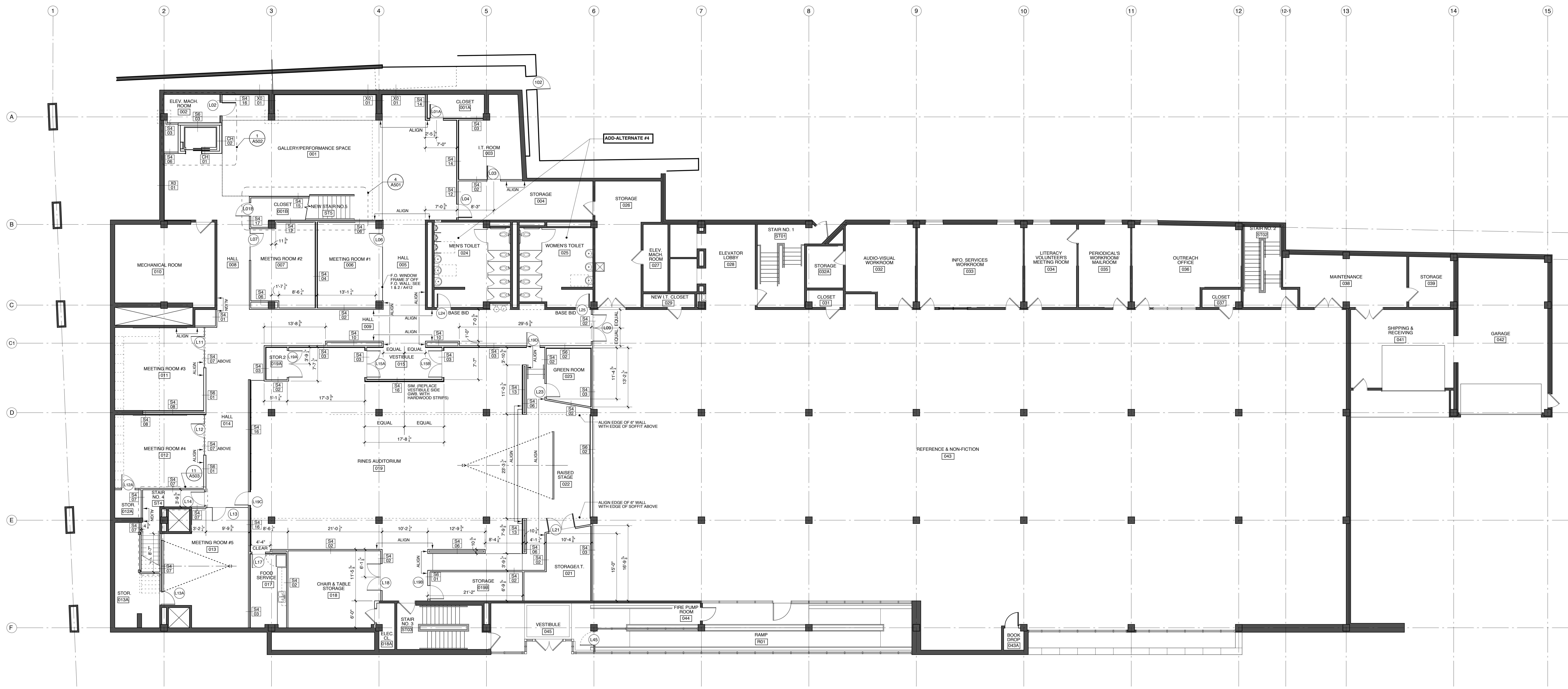
1 LOWER LEVEL DIMENSION PLAN SCALE: 1/8" = 1'-0"
