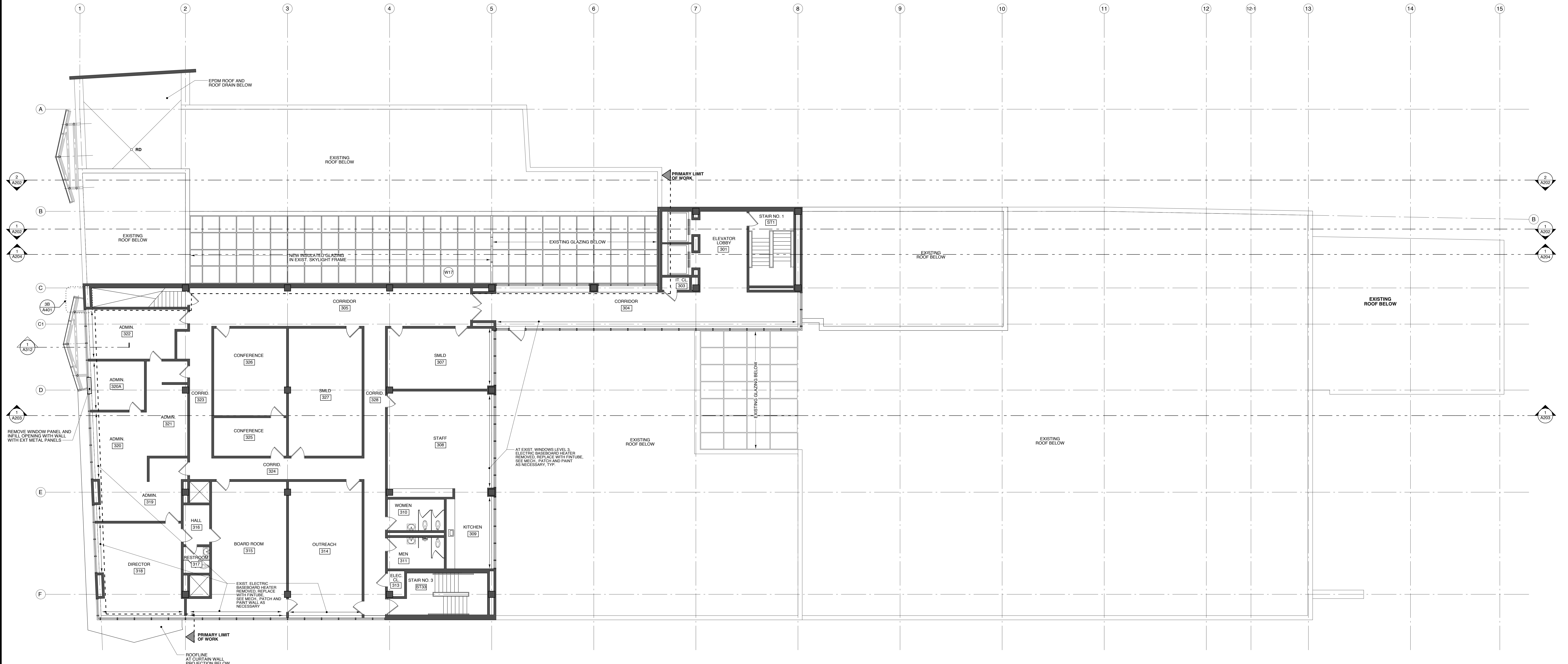
1 LEVEL 3 FLOOR PLAN SCALE: 1/8" = 1'-0"
