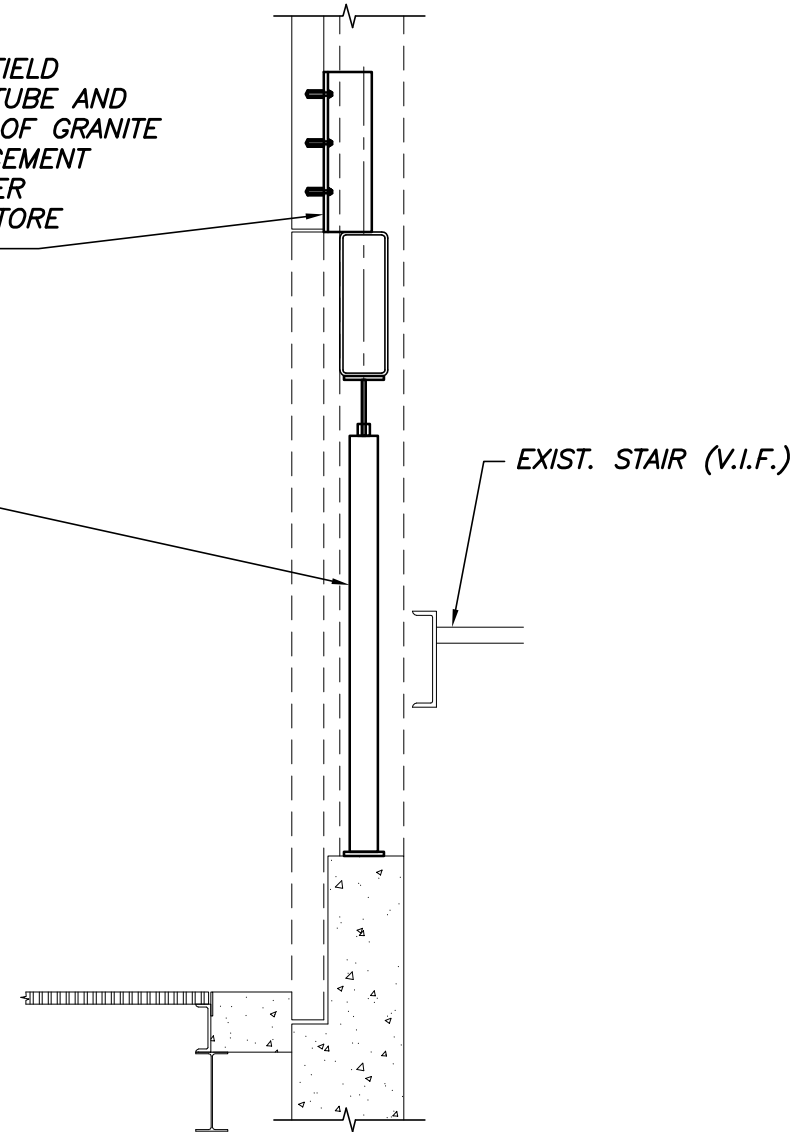
SECTION 1/2"=1'-0"
