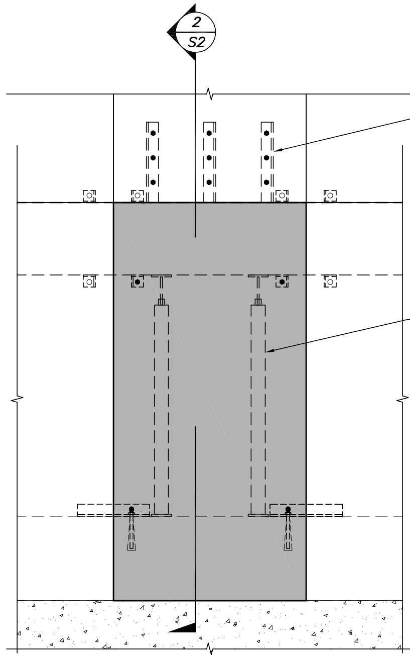
CONCEPTUAL SHORING ELEVATION 1/2"=1'-0"
