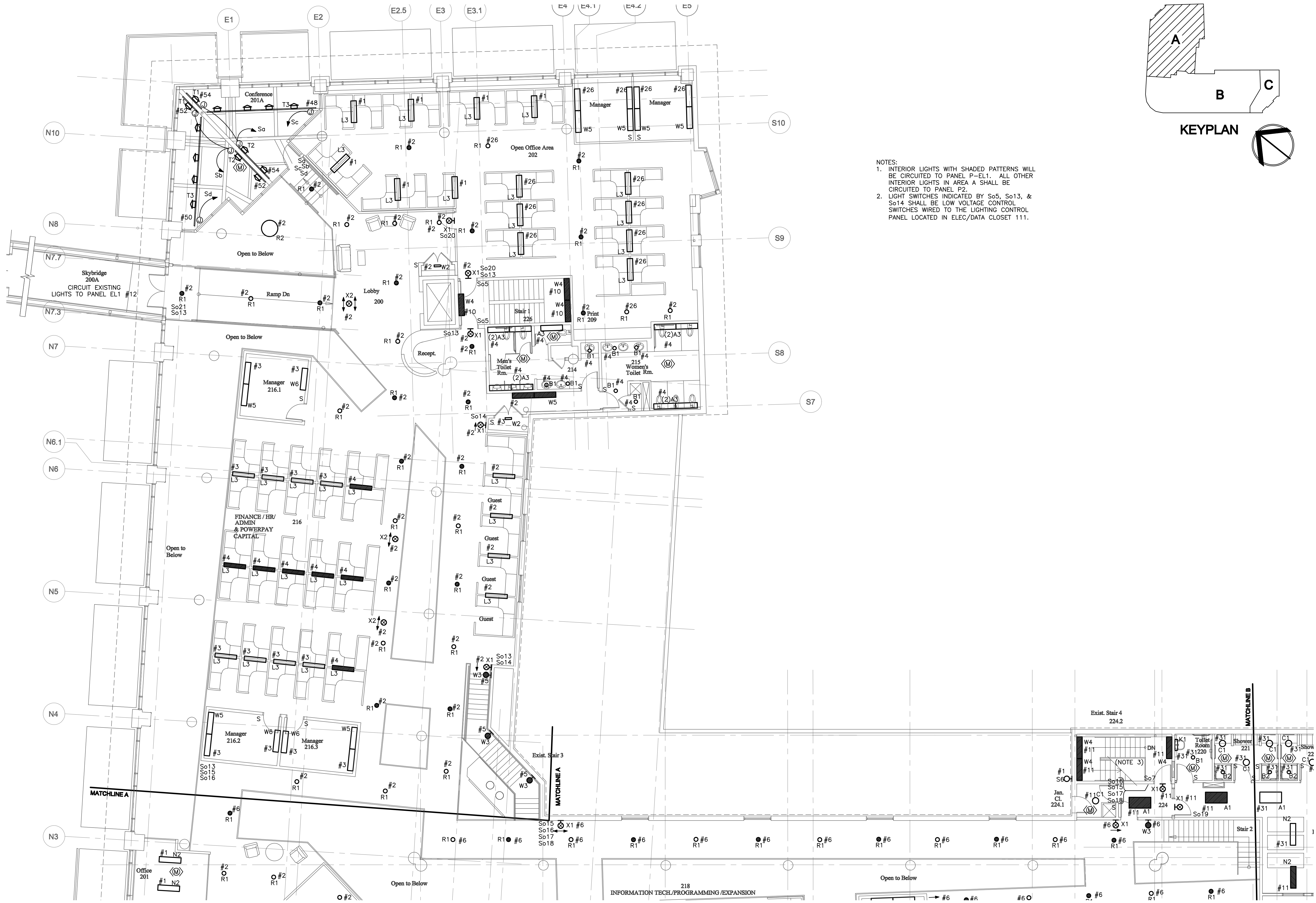
1 SECOND FLOOR LIGHTING PLAN - PART A E2.4 1/8" = 1'-0"
