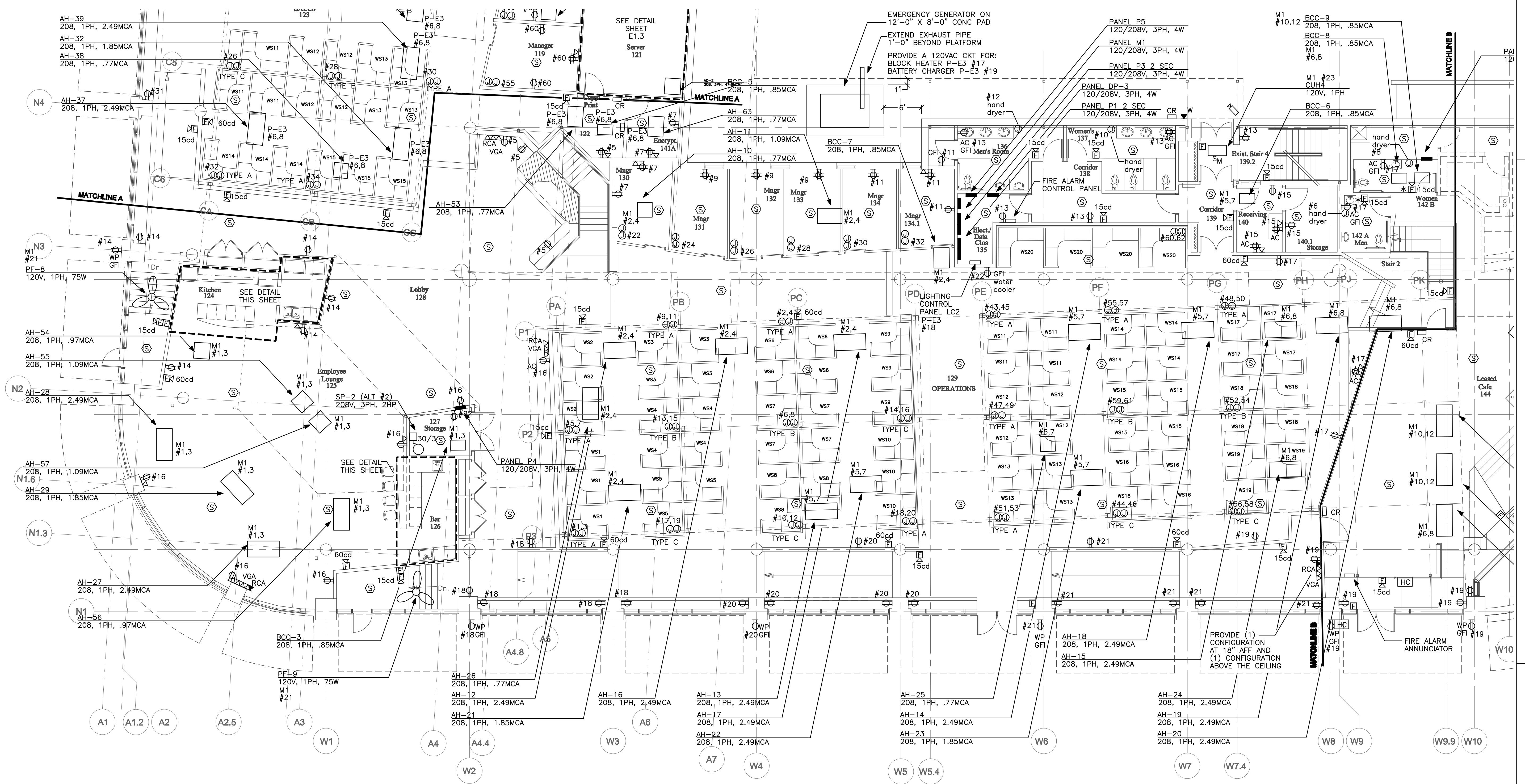
1 FIRST FLOOR POWER PLAN - PART B E1.2 1/8" = 1'-0"
