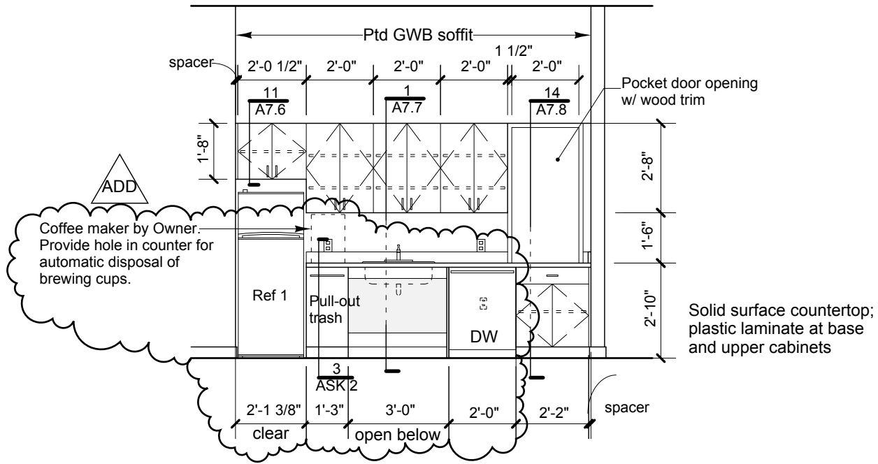
5 COFFEE 209 ELEVATION SCALE: 1/4" = 1'-0"
