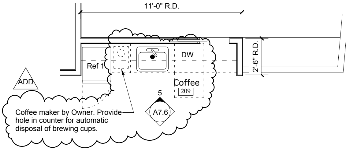
6 COFFEE 209 SCALE: 1/4" = 1'-0"
