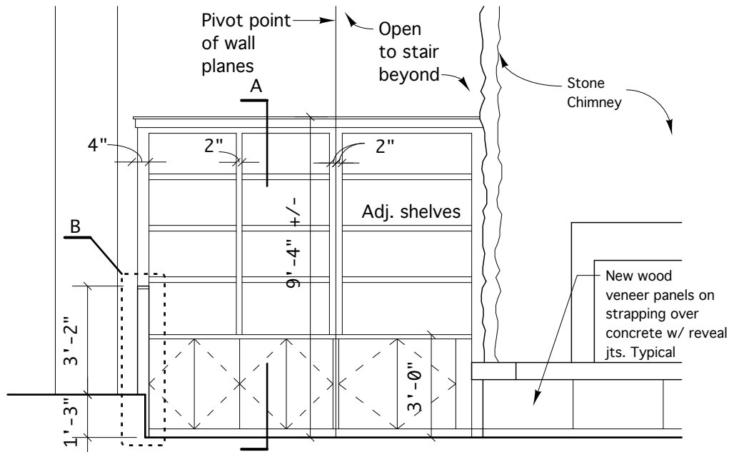
ELEVATION 1 (expanded to show true dimensions)
