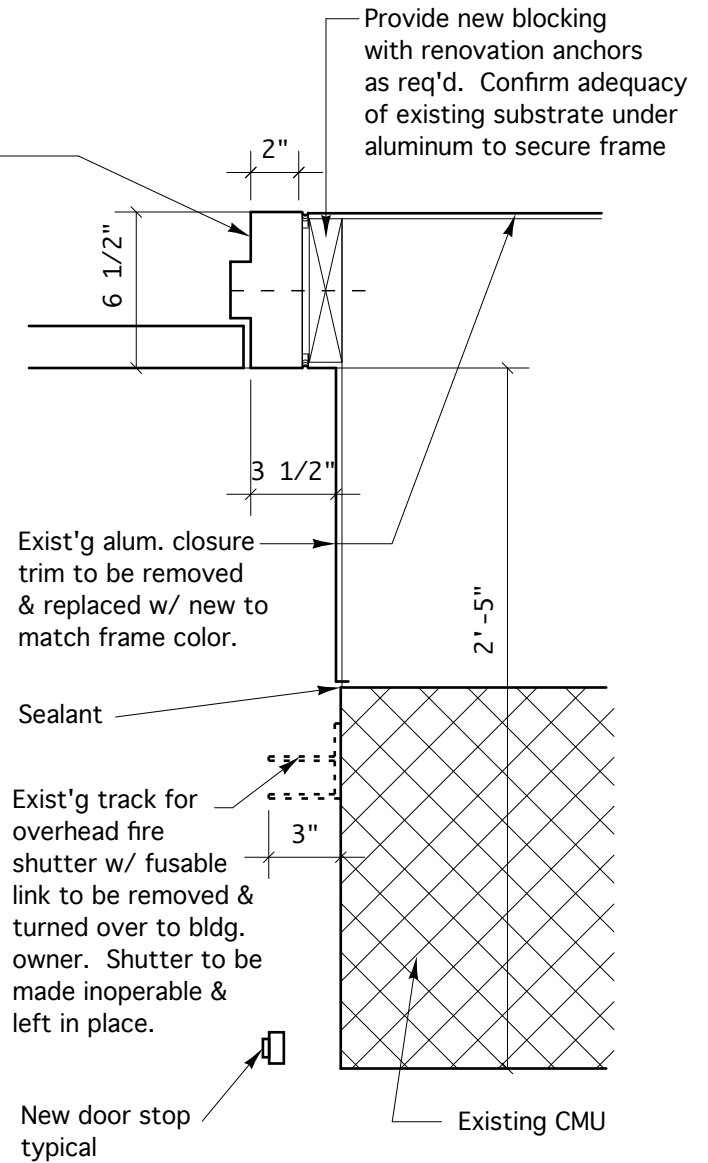
DOOR JAMB DETAIL 1 1/2" = 1'-0"
