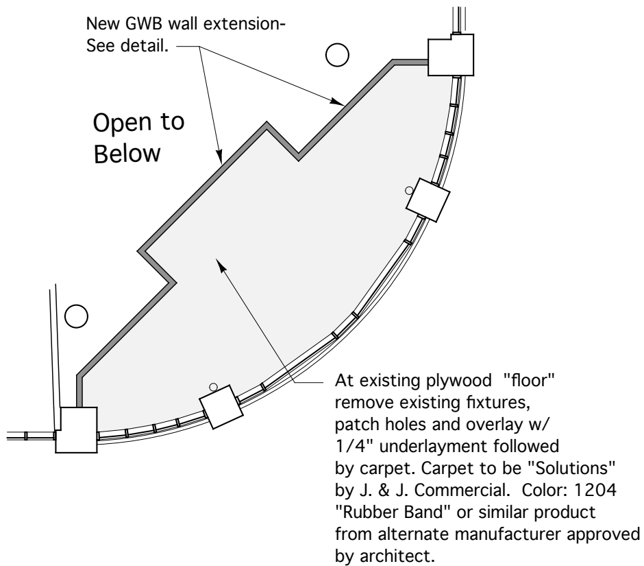
PLAN OF CAFE VESTIBULE AT SECOND FLOOR LEVEL.
