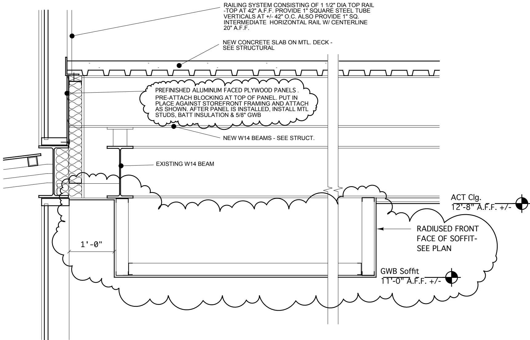
SECTION DETAIL 1
