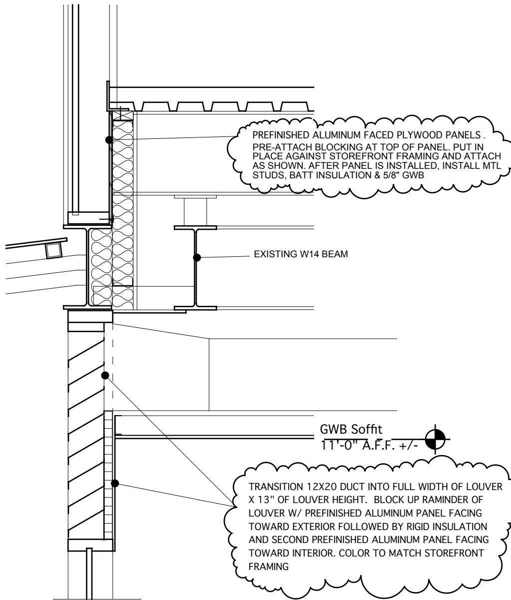
SECTION DETAIL 2
