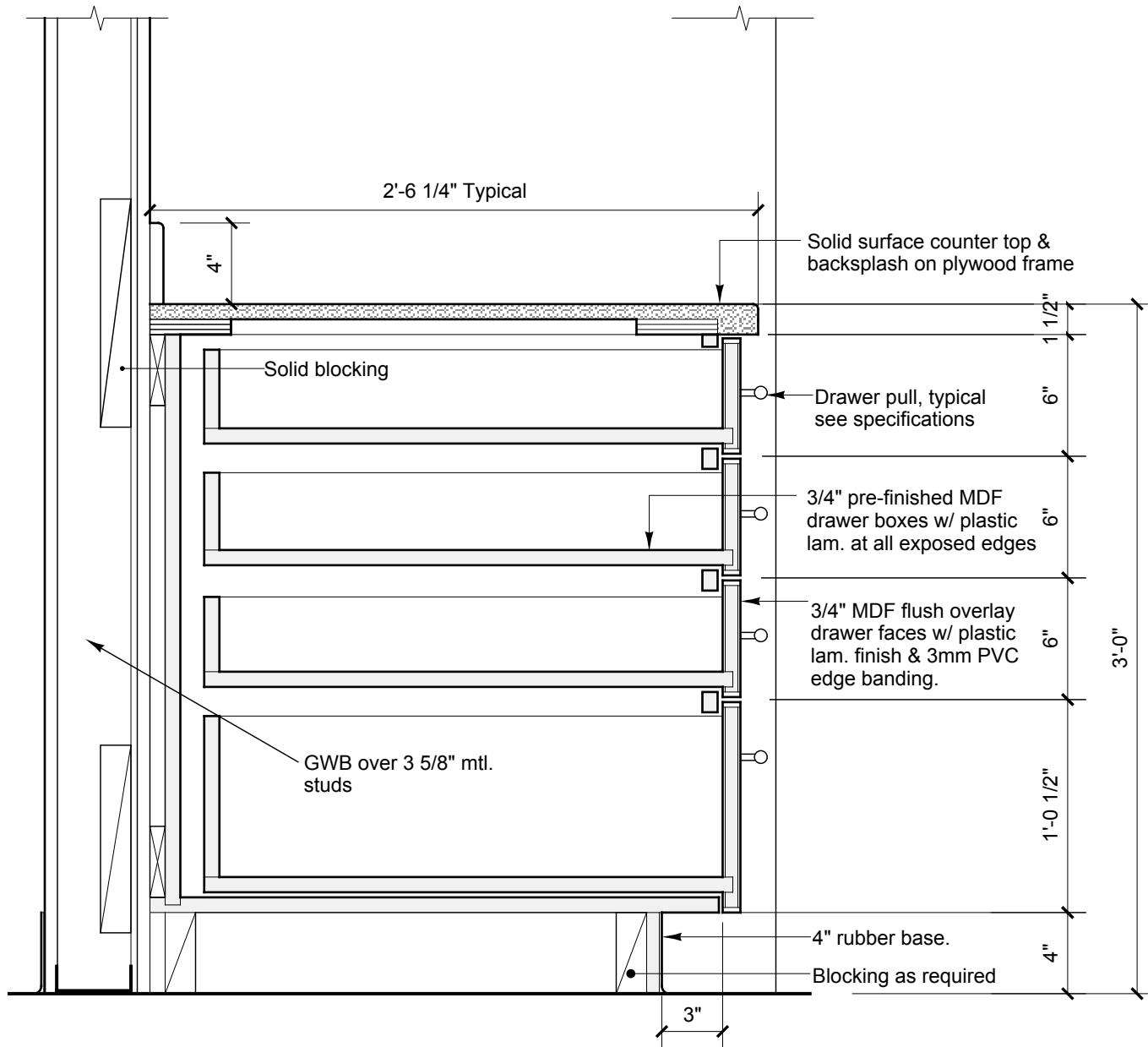
5 EXECUTIVE COFFEE AREA SCALE: 1 1/2" = 1'-0"
