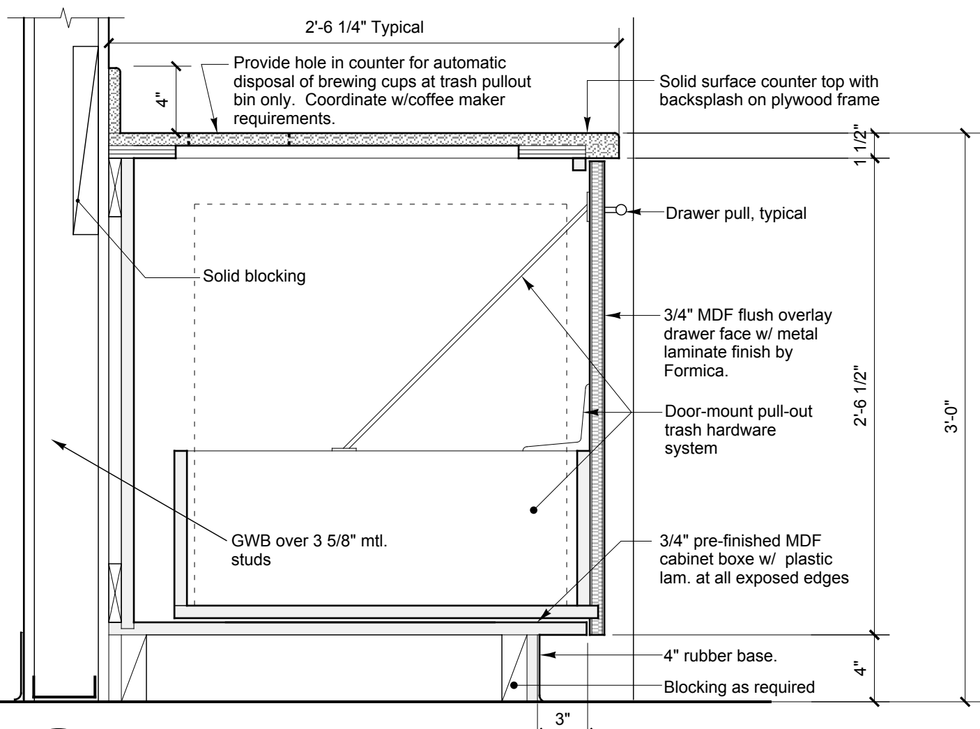
6 SECTION DETAIL AT PULL-OUT CABINET SCALE: 1 1/2" = 1'-0"
