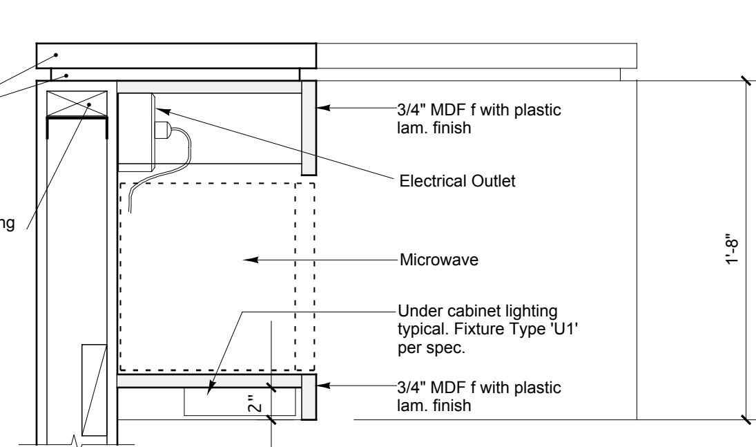
8 SECTION DETAIL AT MICROWAVE SCALE: 1 1/2" = 1'-0"
