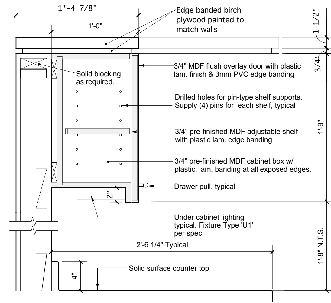
7 SECTION DETAIL AT UPPER CABINET SCALE: 1 1/2" = 1'-0"
