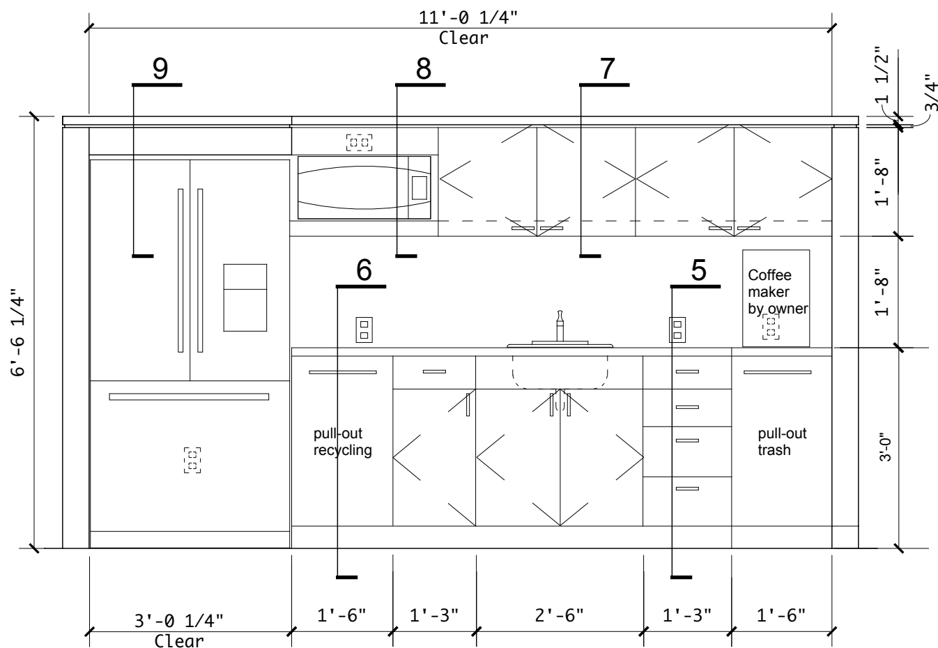
3 EXECUTIVE COFFEE AREA ELEVATION SCALE: 1/2" = 1'-0"
