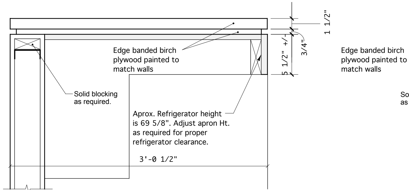
9 SECTION DETAIL AT REFRIGERATOR SCALE: 1 1/2" = 1'-0"
