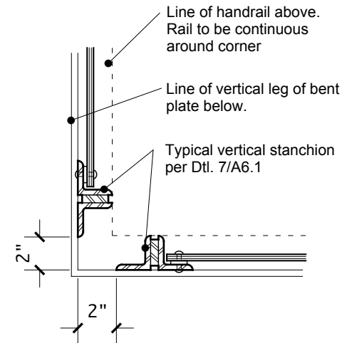
TYPICAL PLAN VIEW 90° INSIDE CORNER RAIL DETAIL
