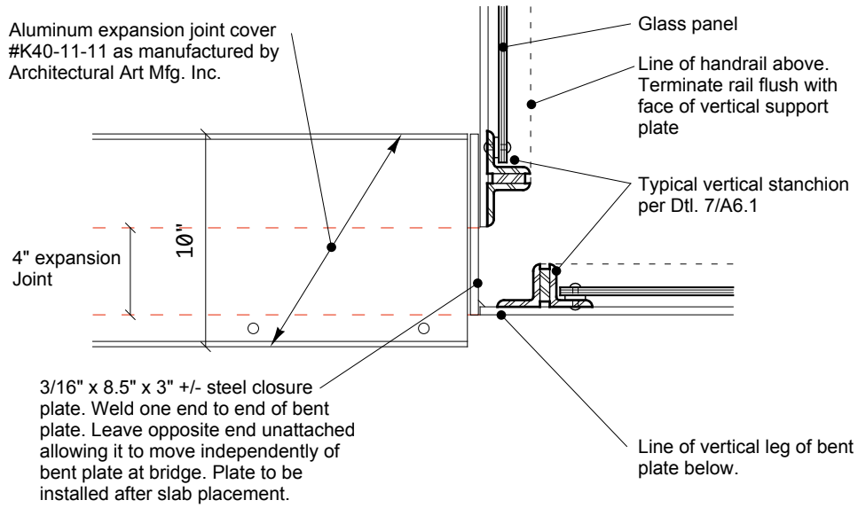
TYPICAL PLAN VIEW RAIL DETAIL FOR 90° CORNER @ EXPANSION JT
