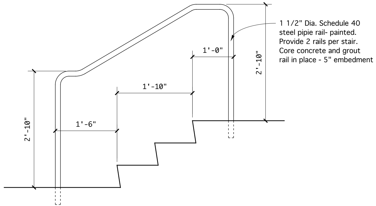
TYPICAL STAIR RAIL DETAIL @ 3 RISER STEPS
