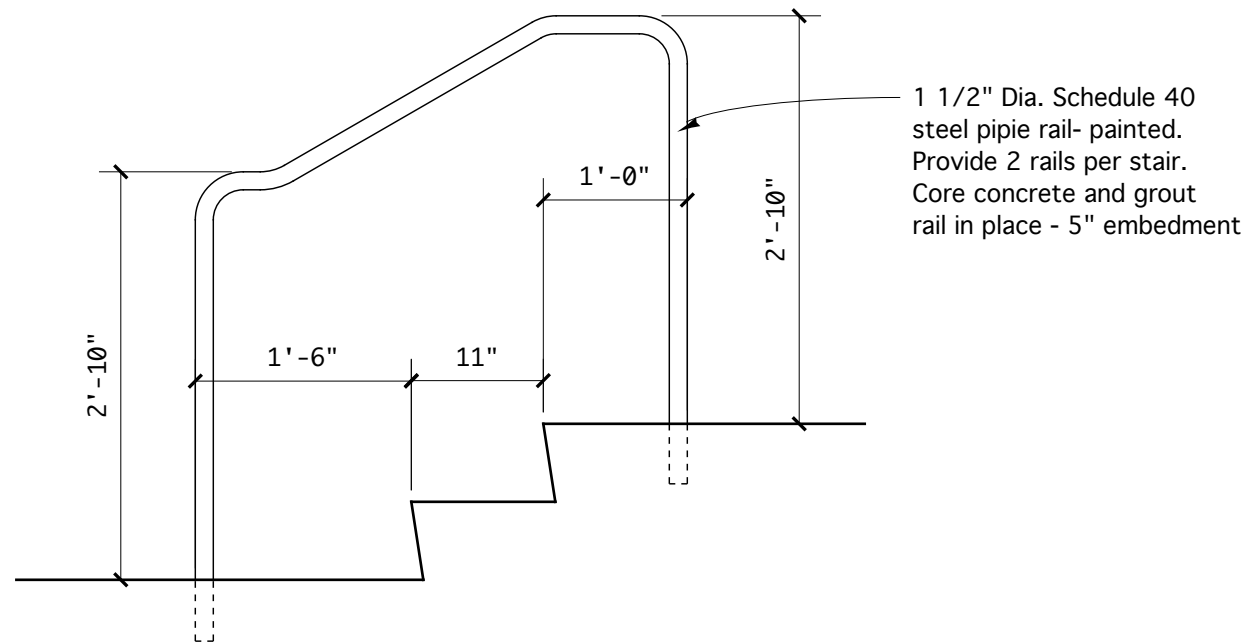
TYPICAL STAIR RAIL DETAIL @ 2 RISER STEPS
