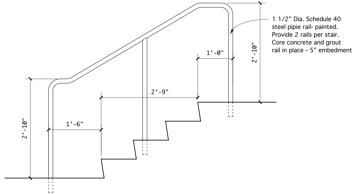
TYPICAL STAIR RAIL DETAIL @ 4 RISER STEPS
