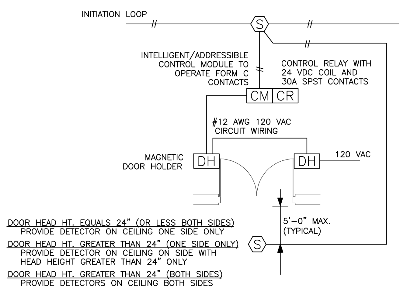
DOOR HOLDER FIRE ALARM INTERFACE WIRING DIAGRAM NOT TO SCALE
